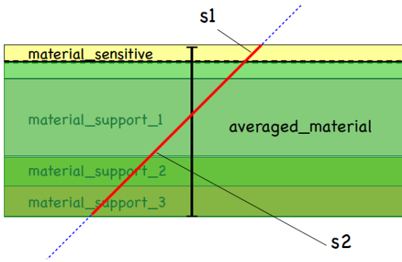
Figure 5. Schematic view of a module that is a part of a tracking detector and how a surface (black dashed line) is placed in the module. s_1 and s_2 are the track segments before and after the surface.
