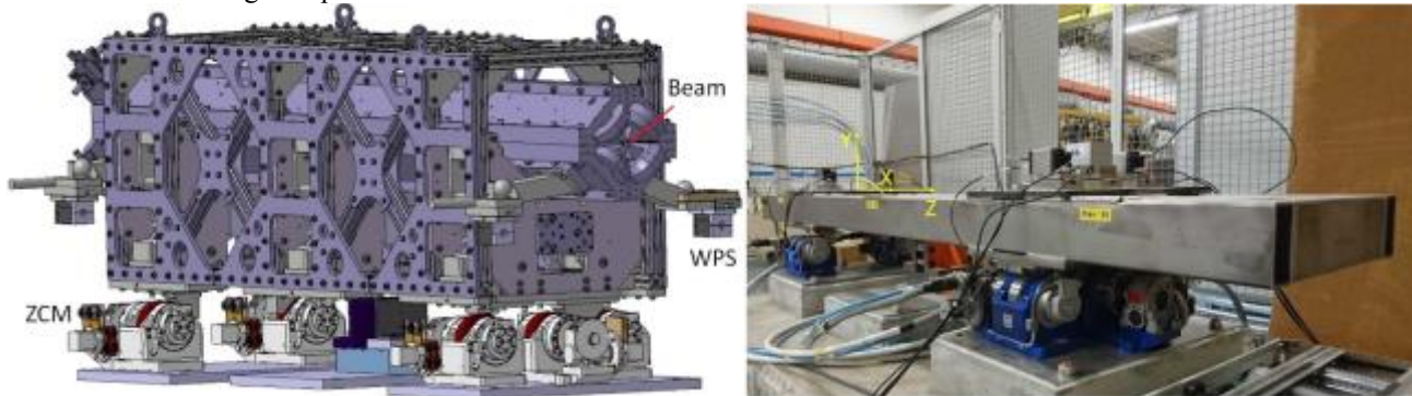
Figure 2: Type 4 MBQ and stabilisation system mounted on cam movers (left) and test setup including ZCMs, follower girder and local coordinate system (right)
