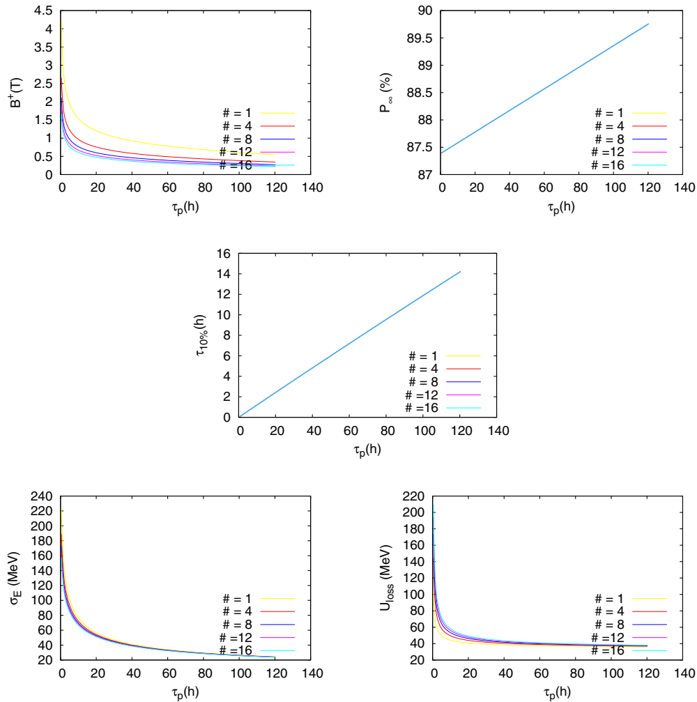
FIG. 3. Parameter values vs. polarization time for different numbers of wigglers units at 45 GeV with N = 6 and L^+ = 1.3 m. Top left: B^+ . Top right: Asymptotic polarization. Center: \tau_{10\%} . Bottom left: Energy spread. Bottom right: Energy lost per turn.
