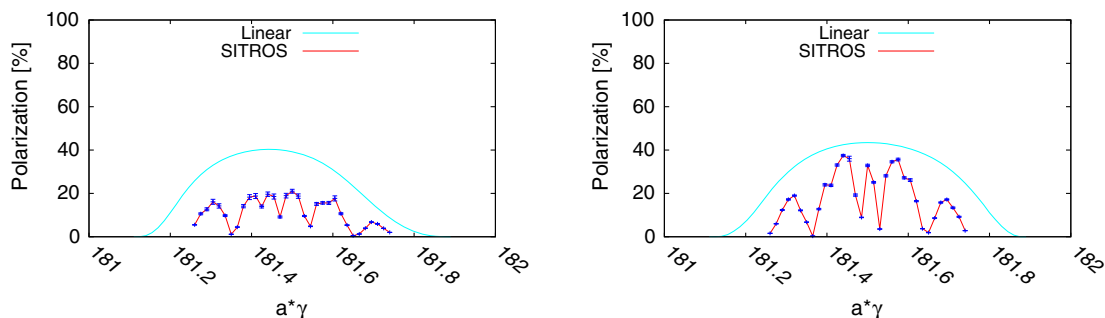
FIG. 11. 60^\circ/60^\circ FODO. Polarization vs. spin tune after orbit is corrected with SVD in presence of BPMs errors. \delta\hat{n}_0 is corrected by 8 3-correctors harmonic bumps (left) or by 8 dispersion-free 5-correctors harmonic bumps (right).
