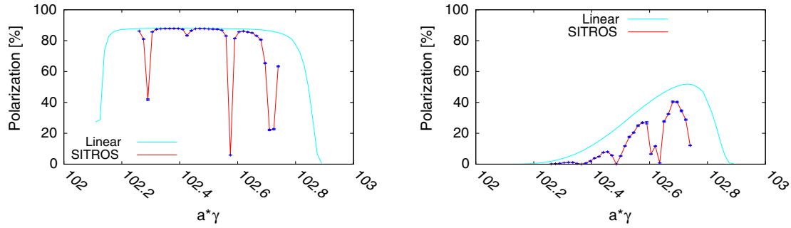
FIG. 13. 90^\circ/90^\circ FODO. Left: Polarization vs. spin tune after orbit is corrected with 1096 correctors with \delta_y^Q = 200 \mu\text{m} and w/o BPMs errors; 4 wigglers with B^+ = 0.7 \text{ T} . Right: adding the BPMs errors.
