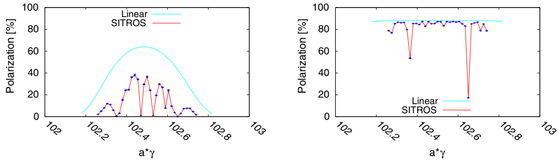
FIG. 6. 60^\circ/60^\circ FODO. Left: Polarization vs. spin tune after orbit is corrected with 1096 correctors with \delta_y^Q = \delta_y^M = 200 \mu\text{m} and 10% BPM calibration error; 4 wigglers with B^+ = 0.7 \text{ T} . Right: adding the correction of \delta\hat{n}_0 through harmonic bumps.
