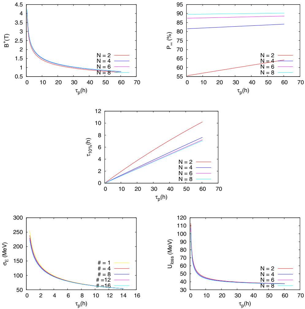
FIG. 2. Parameter values vs. polarization time for one wiggler at 45 GeV for various values of N . Top left: B^+ . Top right: Asymptotic polarization. Center: \tau_{10\%} . Bottom left: Energy spread. Bottom right: Energy lost per turn.
