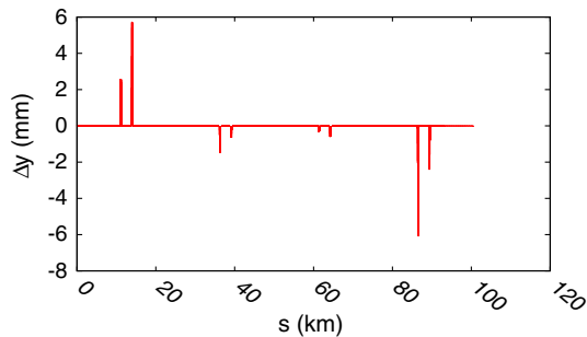
FIG. 10. Vertical closed orbit change due to the 8 3-correctors harmonic bumps for the 80 GeV case.
