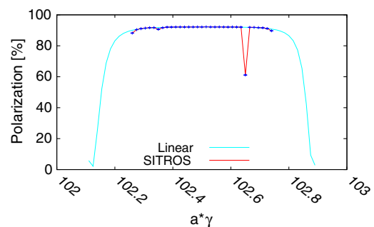
FIG. 5. Polarization vs. spin tune after orbit is corrected by using all 1096 correctors with \delta_y^0 = 200 \mu\text{m} , w/o BPMs errors and in presence of 4 wigglers with B^+ = 0.7 T. 60°/60° FODO.
