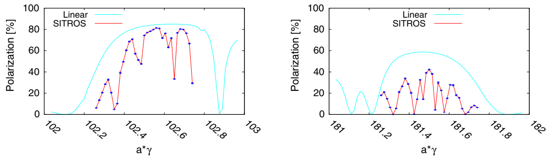
FIG. 14. 90^\circ/90^\circ FODO. Left: Polarization vs. spin tune after orbit and \delta\hat{n}_0 correction with \delta_y^Q = \delta_y^M = 200 \mu\text{m} and 10% BPMs calibration error; 4 wigglers with B^+ = 0.7 \text{ T} (45 GeV). Right: Polarization vs. spin tune after orbit and \delta\hat{n}_0 correction with \delta_y^Q = \delta_y^M = 200 \mu\text{m} and 10% BPMs calibration error, no wigglers (80 GeV).
