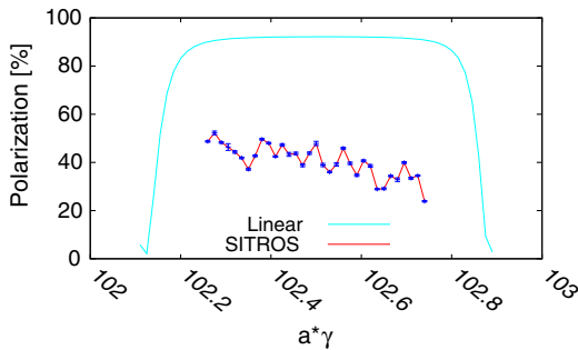
FIG. 7. Polarization vs. spin tune after orbit is corrected with 1096 correctors in presence of BPMs errors with B^+ = 3.9 \text{ T} .
