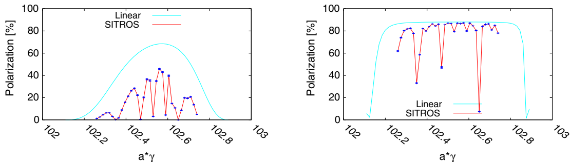
FIG. 8. 60^\circ/60^\circ FODO. Left: Polarization vs. spin tune after orbit is corrected with 110 correctors with \delta_y^Q = \delta_y^M = 200 \mu\text{m} and 10% BPM calibration error; 4 wigglers with B^+ = 0.7 \text{ T} . Right: adding the correction of \delta\hat{n}_0 through orbit bumps.
