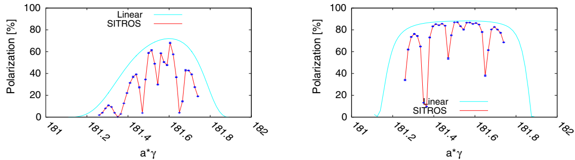
FIG. 9. 60^\circ/60^\circ FODO. Left: Polarization vs. spin tune after orbit is corrected with 1096 correctors with \delta_y^0 = 200 \mu\text{m} and no BPMs errors. Right: adding the correction of \delta\hat{n}_0 through orbit bumps.
