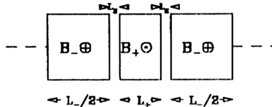
FIG. 1. LEP polarization wiggler (figure from [18]).
