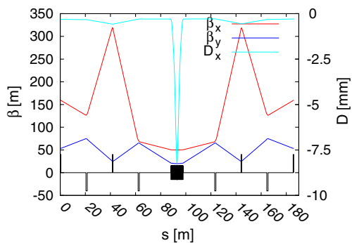
FIG. 4. Twiss and dispersion functions in the wiggler section with B^+ = 0.7 T. The Twiss functions are practically unchanged; the peak |D_x| (and orbit deviation) is 8 mm.
