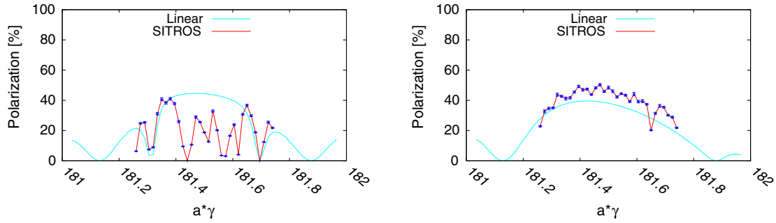
FIG. 12. Polarization vs. spin tune after orbit is corrected with SVD in presence of BPMs errors and \delta\hat{n}_0 is corrected with 5-correctors harmonic bumps. Left: Q_s = 0.3 . Right: Q_s = 0.9 .
