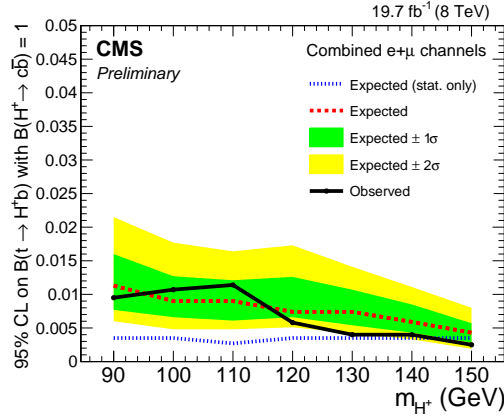
Figure 2: Observed upper limits on combined e+\mu channel with expected limits including all systematic uncertainties. The limits with statistical uncertainty only are overlaid in blue dots to show the effect of systematic uncertainties.
