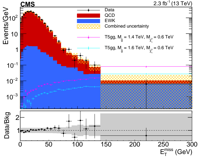
Figure 3: Measured E_T^{\text{miss}} distribution in comparison with the background prediction. The four bins with E_T^{\text{miss}} \geq 100 \text{ GeV} constitute the signal region, and the E_T^{\text{miss}} < 100 \text{ GeV} bins serve mainly to normalize the background. The systematic uncertainty on the background prediction and the ratio of the data to the prediction are also shown. The last bin includes all events with E_T^{\text{miss}} \geq 140 \text{ GeV} , but for normalization by bin width, the bin is taken to be from 140 \leq E_T^{\text{miss}} < 300 \text{ GeV} . The distributions for two signal model points are overlaid for comparison.
