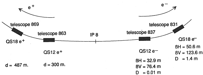
Fig. 1 : Synchrotron Light Monitor locations.
