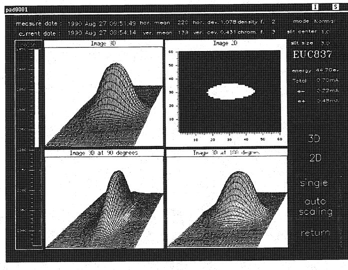
2D and 3D image plots and profiles of a circulating beam displayed on a workstation.
