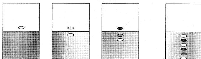
Fig. 5 : "Burst mode": The top zone is the image area on which the synchrotron light is imaged. The shaded zone is the memory area. Between successive light pulses, controlled by the fast shutter, the stored profiles are shifted down to the memory area. At the end of the process up to eighteen profiles (six illustrated) are stored in the memory area of the CCD.
