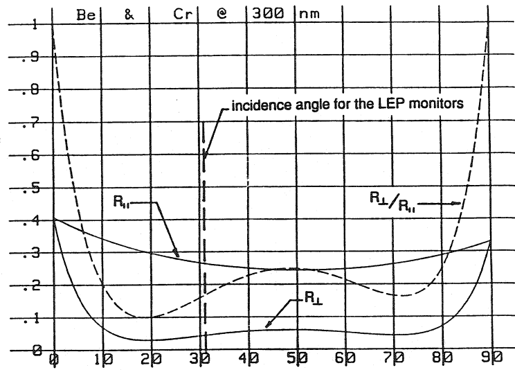
Reflection coefficients for the vertical and horizontal polarization components of the synchrotron radiation and their ratio as a function of the incidence angle on the beryllium mirror.
