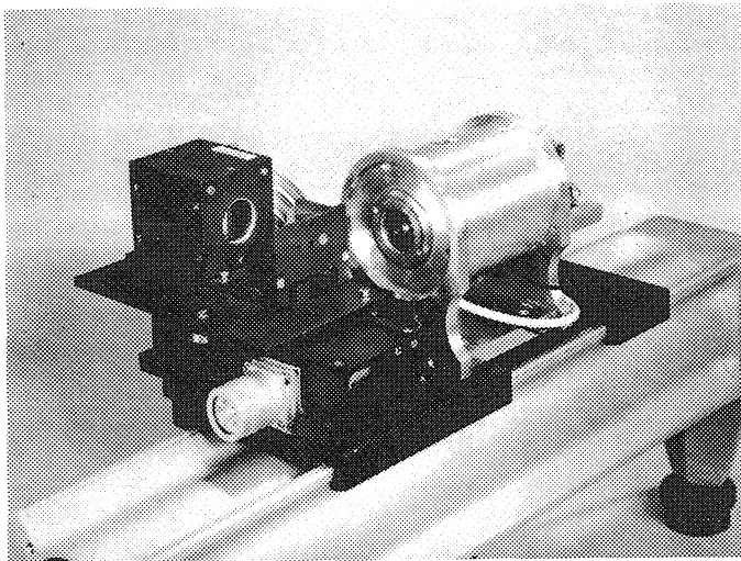
The two detectors - the normal CCD camera (left) and the UV converter/shutter with its CCD chip.
