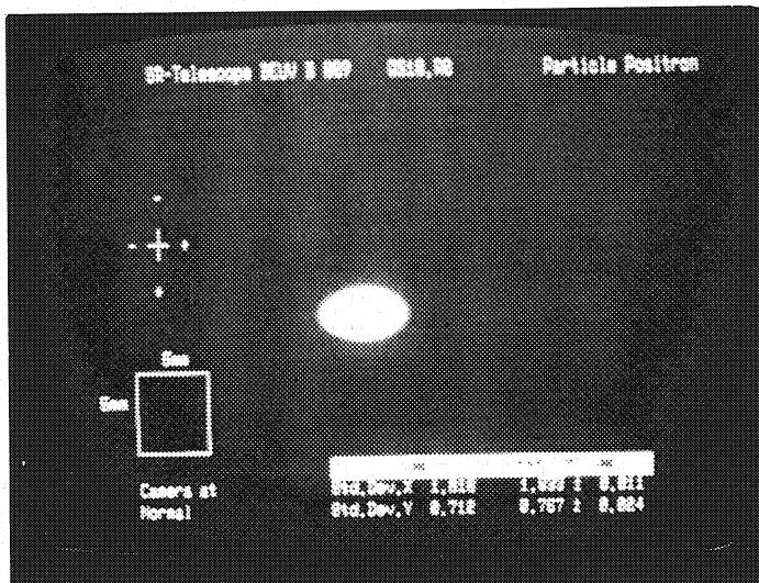
A circulating beam as seen on the TV display in the PCR. The telescope location, particle type and standard deviation of the beam sizes (last and averaged measurements) are also displayed.
