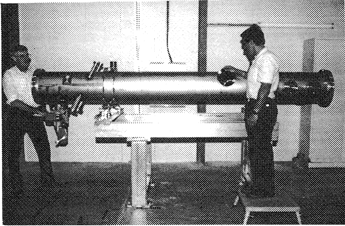
The telescope ready for installation in the LEP tunnel
