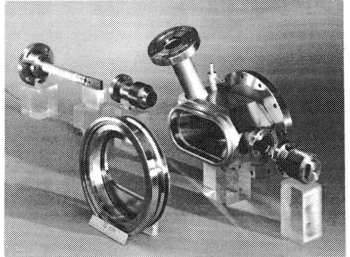
Components of the light extraction system. The beryllium mirror can be seen at the top left hand side.
