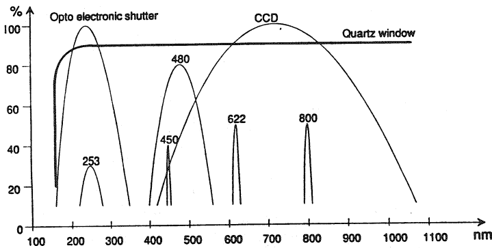
Filters and detectors wavelength characteristics. The light transmission or sensitivity for each element in the system is plotted against wavelength in nanometers.
