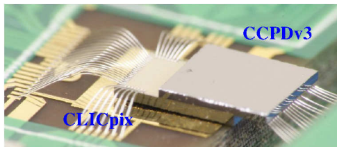
(b) Assembly on readout board
