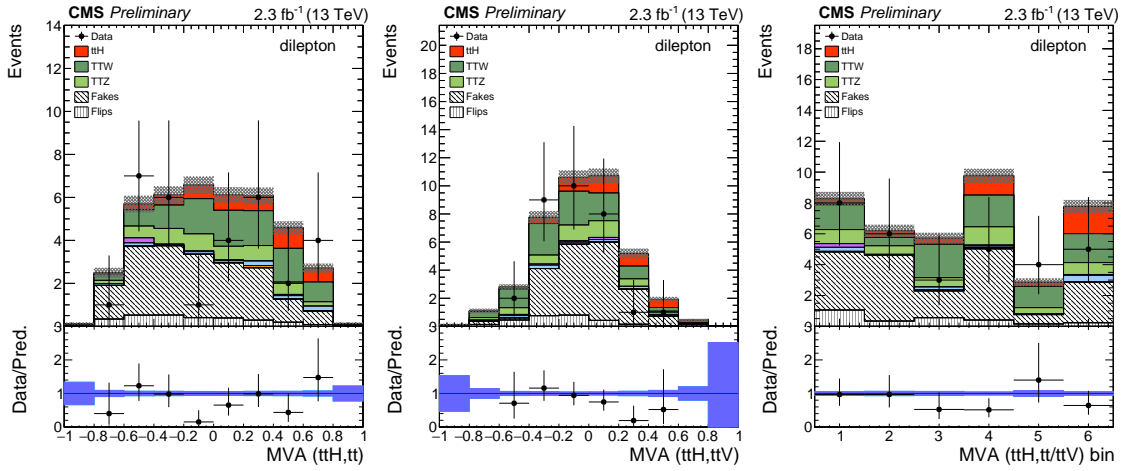
Figure 4: Distributions of the BDT kinematic discriminants and result of their combination in the bins used for signal extraction, for the two same-sign lepton selection inclusive in lepton flavor. Pre-fit distributions are shown. Uncertainties are statistical only.
