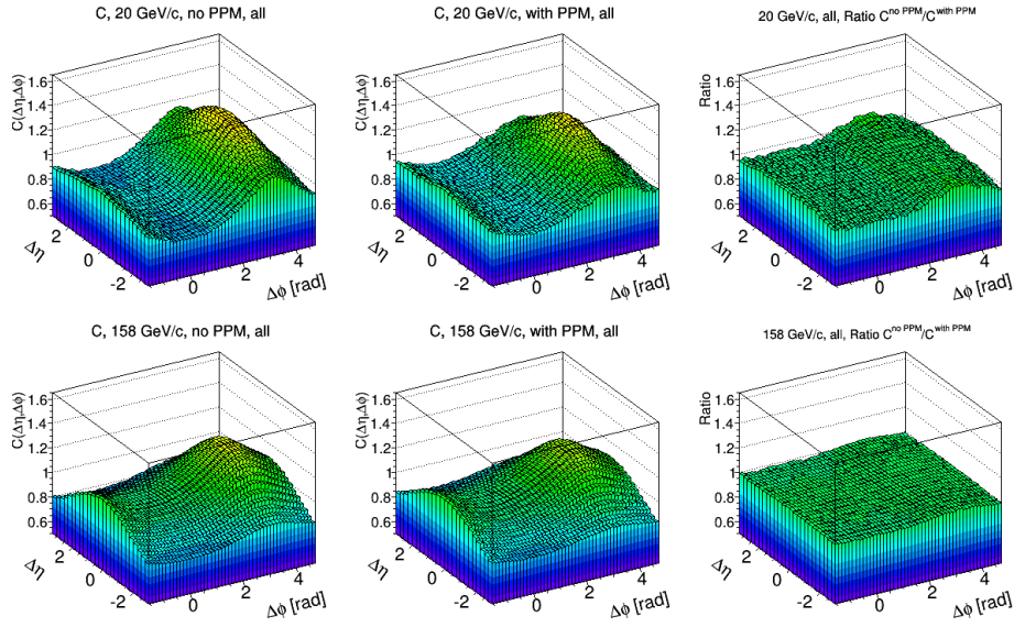
Figure 10: NA61/SHINE detector acceptance effects studied with the Epos [21] model. Left plots show correlation functions in almost complete acceptance (only p_T < 1.5 GeV/c cut was applied), middle plots show correlation functions in NA61/SHINE acceptance, right plots – ratios of these two. Top row shows results for 20 GeV/c, bottom row for 158 GeV/c.
