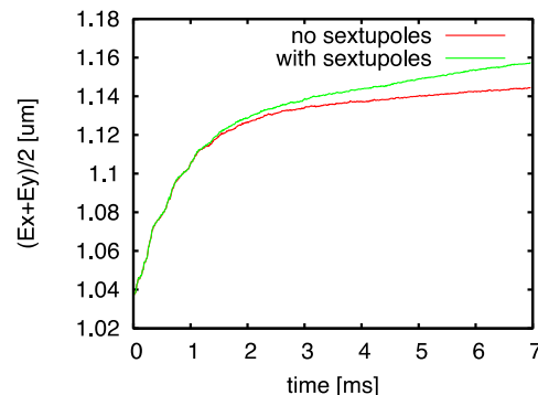
Figure 10: Emittance evolution vs. time, assuming no sextupolar errors in the lattice and with errors. Simulations at 160 MeV, N_p=260 \times 10^9 , WP (4.33,4.55).
