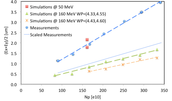
Figure 4: Semi-sum of the normalized rms emittances versus intensity. Blue points: measurements [4]; blue line: measurements slope scaled by 2; green and orange: simulations at 160 MeV injection energy, for two working points; red: simulations at 50 MeV, as in Fig. 2.
