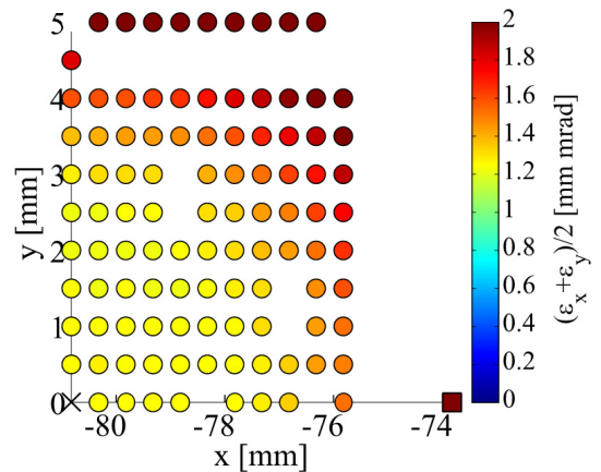
Figure 5: The simulated final emittance (semi-sum of the normalized rms emittances) after 10 ms tracking with respect to the injection offset in x and in y [9]. The beam intensity is N_p=3.42e12 and the bare tune is (4.43, 4.60).
