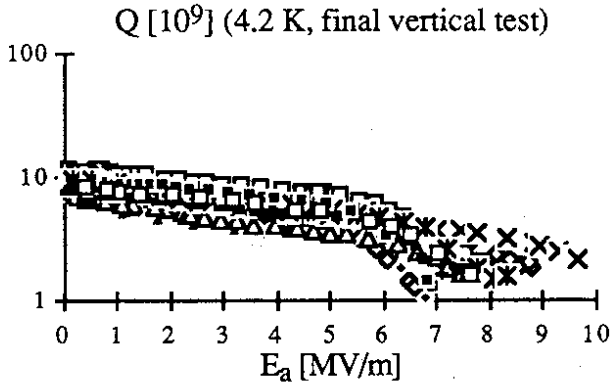
Fig. 1 Q value vs accelerating field for LEP type Nb/Cu cavities.
