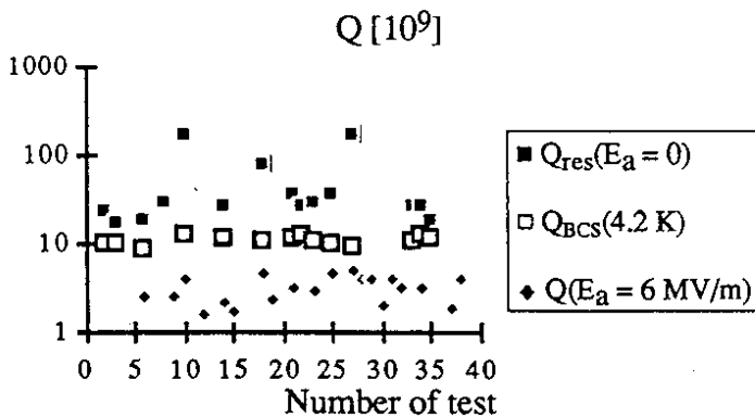
Fig. 2 Q values vs test number for all RF tests performed.
