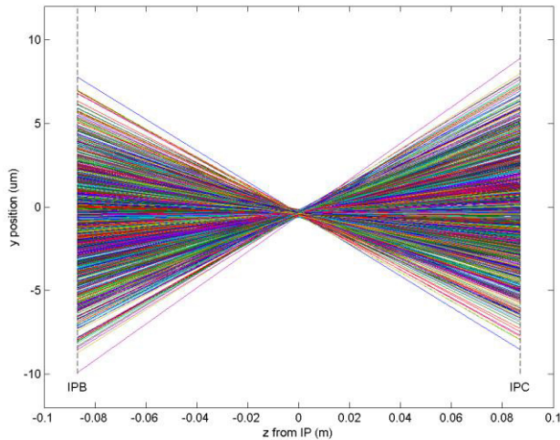
Figure 6: Vertical bunch position y , obtained for each trigger by linearly interpolating the measured beam positions at IPB and IPC, versus longitudinal distance z from the IP.
