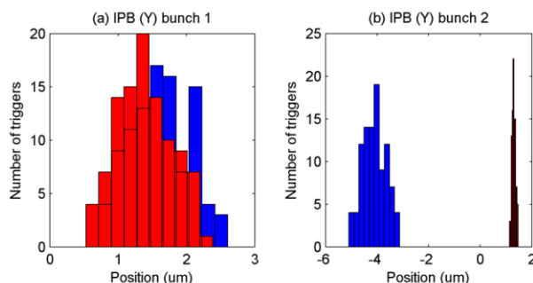
Figure 4: Distribution of the vertical position of (a) bunch 1 and (b) bunch 2 in IPB with (red) and without (blue) application of the IP feedback correction.
