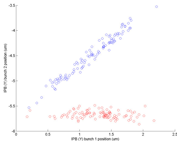
Figure 5: Vertical position for bunch 2 versus bunch 1 in IPB with (red) and without (blue) application of the IP feedback correction.
