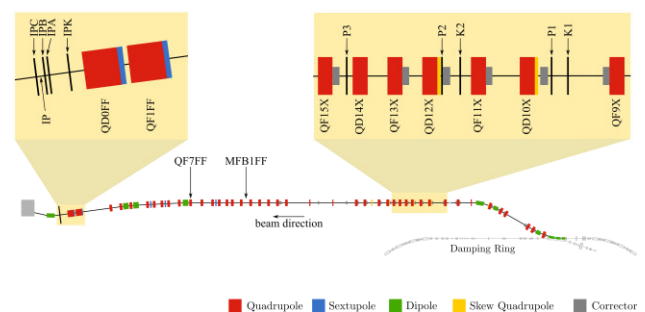
Figure 1: Layout [5] of the ATF2 extraction and final focus beamline with the FONT regions zoomed in.
