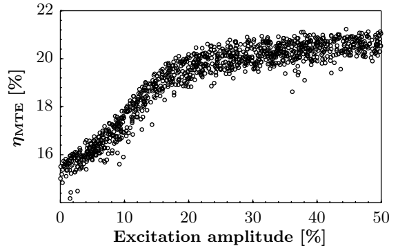
Figure 10: Dependency of the splitting efficiency on the excitation amplitude of the transverse damper (in % of the maximum amplitude). An amplitude of at least 20% is required to achieve proper splitting efficiency.
