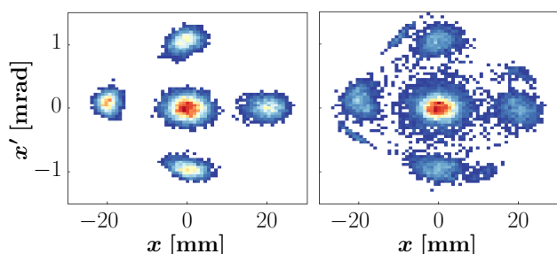
Figure 3: Simulated horizontal phase space portraits at the end of the splitting process in the absence of a tune ripple (left) and with a ripple amplitude corresponding to the maximum measured current ripple on the PFW circuits (right). The efficiency of the splitting process is clearly reduced in the latter case.
