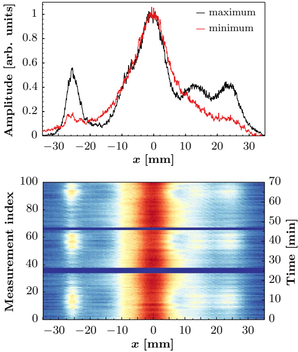
Figure 1: Top: Comparison between good and bad splitting efficiency based on measured horizontal profiles. Bottom: Waterfall representation of multiple measured horizontal profiles, with the colour scale corresponding to the amplitude of the data shown in the image at the top. Each measurement was recorded on a different cycle and clear oscillations of the beamlets' intensities are visible.
