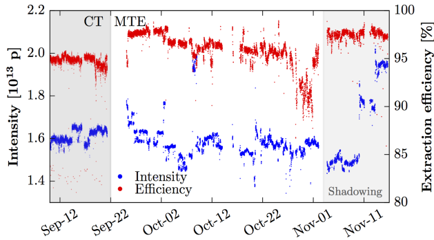
Figure 9: Evolution of the PS proton intensity measured prior to extraction and of \eta_{\text{ext}} during the 2015 MTE run. Operation with CT and the period using the shadowing configuration are highlighted in grey.
