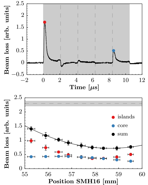
Figure 7: Top: Signal of the fast BLM16. The grey area indicates a duration of five turns, with the dashed lines being separated by one turn. The red and the blue circles correspond to the maximum beam loss occurring during the extraction of the islands and the core, respectively. Bottom: Dependency of beam loss on the position of SMH16 for an angle of 0 mrad. Red and blue circles correspond to the losses of the islands and the core, respectively, and the black circles represent their sum. Error bars describe the standard deviation obtained over 10 consecutive measurements. The dashed line and the grey band indicate mean value and standard deviation of losses for the nominal septa settings.
