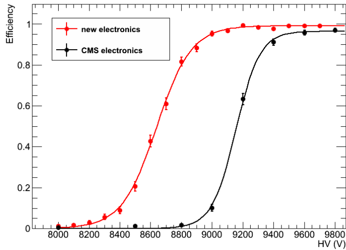
Figure 5. Left: block diagram of INFN amplifier where R1 is the input impedance resistance. C1 \ll C2 and R1 \ll R2 are the conditions for the circuit to work properly. Right: efficiency plateaus for the cases of the standard CMS RPC front-end electronics and new INFN prototype electronics. A lower charge crossing the RPC gap is indicated by the shift of the plateau toward lower voltages leading to an improved rate capability of the RPC.
