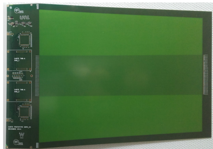
Figure 7. Picture of a strip board designed for a RE1/1 station using 16-channel PETIROC ASICs and 25 ns TDC.
