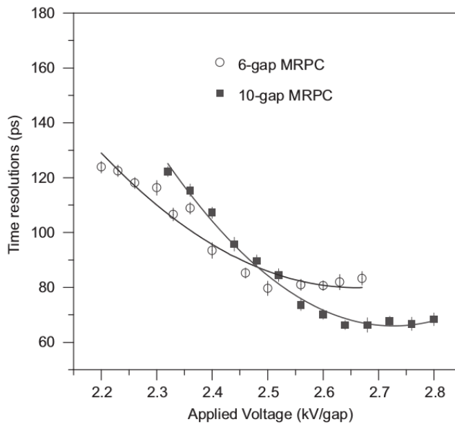
Figure 10. Structure of 6-gap (top) and 10-gap (center) resistive plate chambers from Tsinghua University. Time resolution of 6-gap and 10-gap resistive plate chambers (bottom) as a function of high voltage at an incoming muon rate of 1.2 \text{ kHz/cm}^2 .
