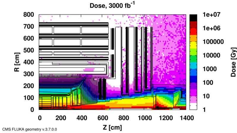
Figure 1. Absorbed dose in the CMS cavern after an integrated luminosity of 3000 fb -1 . R is the transverse distance from the beamline and Z is the distance along the beamline from the Interaction Point at Z=0.
