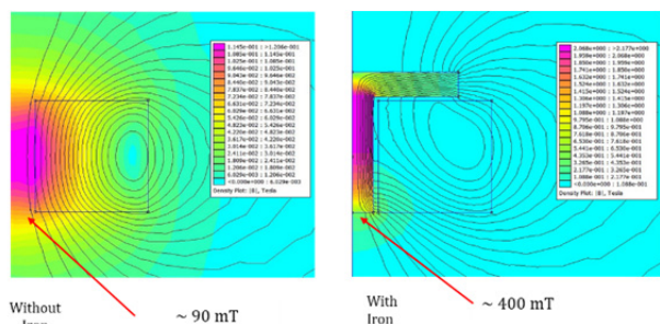
Figure 4: Field lines before and after the insertion of iron core inside the coil to enhance the magnetic field \sim a factor 4 on the sample.
