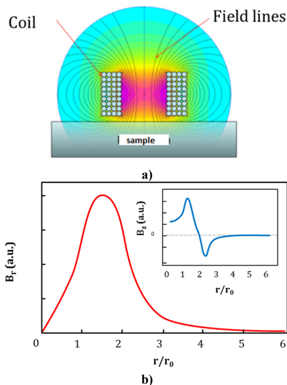
Figure 1: a) Field repartition for a r_0 diameter coil. b) Curve shows the radial repartition 200 \mu\text{m} away from the coils (approximate position of the sample is expected to be closer to the coil: \sim 60 \mu\text{m} ). Inset shows the z component of field behavior.
