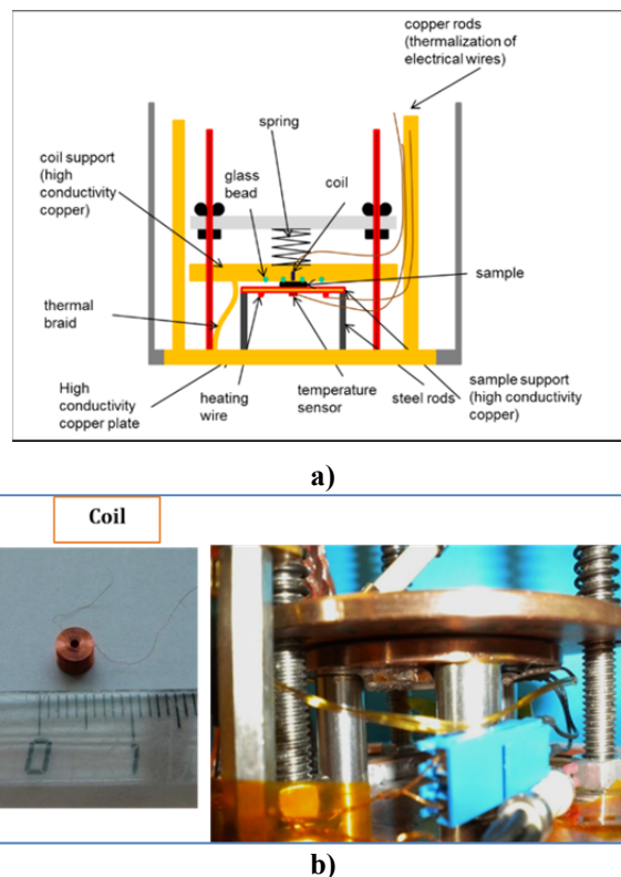
Figure 2: a) Schematic of the local magnetometry facility at Saclay, b) Details of the coil and sample holder.
