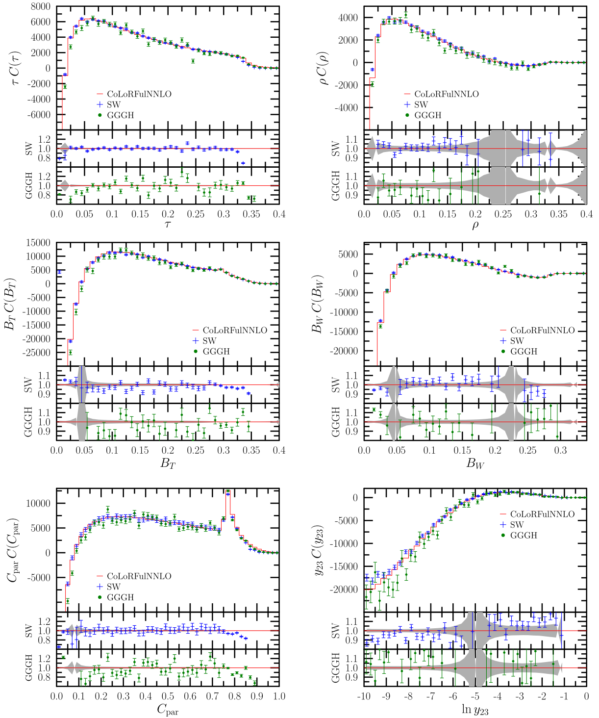
FIG. 4. The OC(O) coefficients of the thrust, heavy jet mass, total and wide jet broadening, C -parameter and two-to-three jet transition variable y_{23} distributions. Lower panels show the ratio of the (updated but unpublished—see text) predictions of Ref. [6] (SW) and EERAD3 [96] (GGGH) to CoLoRFulNNLO (this work). The shaded bands on the lower panels represent the relative statistical uncertainties of our predictions due to Monte Carlo integrations.
