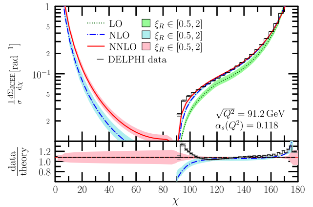
FIG. 5. The distribution of jet cone energy fraction (JCEF) at LO, NLO and NNLO accuracy in perturbative QCD. The bands represent the variation of the renormalization scale in the range \xi_R = \mu/\mu_0 \in [0.5, 2] around the central value of \mu_0 = \sqrt{Q^2} . The lower panel shows the relative scale dependence at NNLO accuracy.
