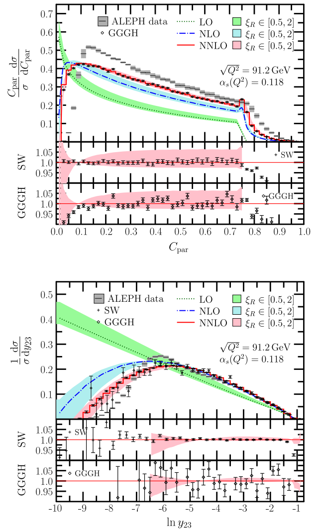
FIG. 3. Same as Fig. 1 for the C -parameter ( C_{\text{par}} ) and the two-to-three jet transition parameter ( y_{23} ) in the Durham clustering algorithm.
