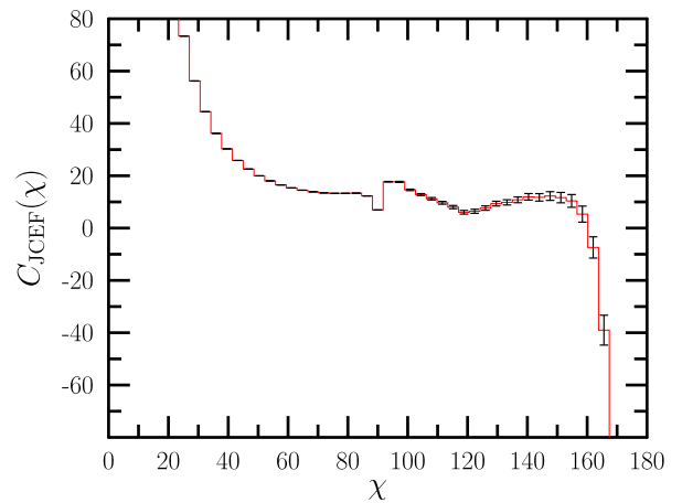
FIG. 6. The distribution of the NNLO coefficient for jet cone energy fraction (JCEF). The error bars represent the statistical uncertainty of the Monte Carlo integrations.
