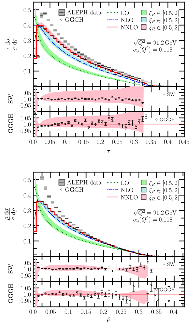
FIG. 1. Perturbative predictions for the thrust ( \tau \equiv 1 - T ) and heavy jet mass ( \rho ) distributions at LO, NLO and NNLO accuracy. The bands represent the renormalization scale uncertainty of our predictions corresponding to the range \xi_R \in [0.5, 2] around the central value of \mu_0 = \sqrt{Q^2} . The lower panels show the ratio of the (updated but unpublished—see text) predictions of Ref. [6] (SW) and EERAD3 [96] (GGGH) to CoLoRFulNNLO (this work). The bands on the lower panels show the relative scale uncertainty of our NNLO results.
