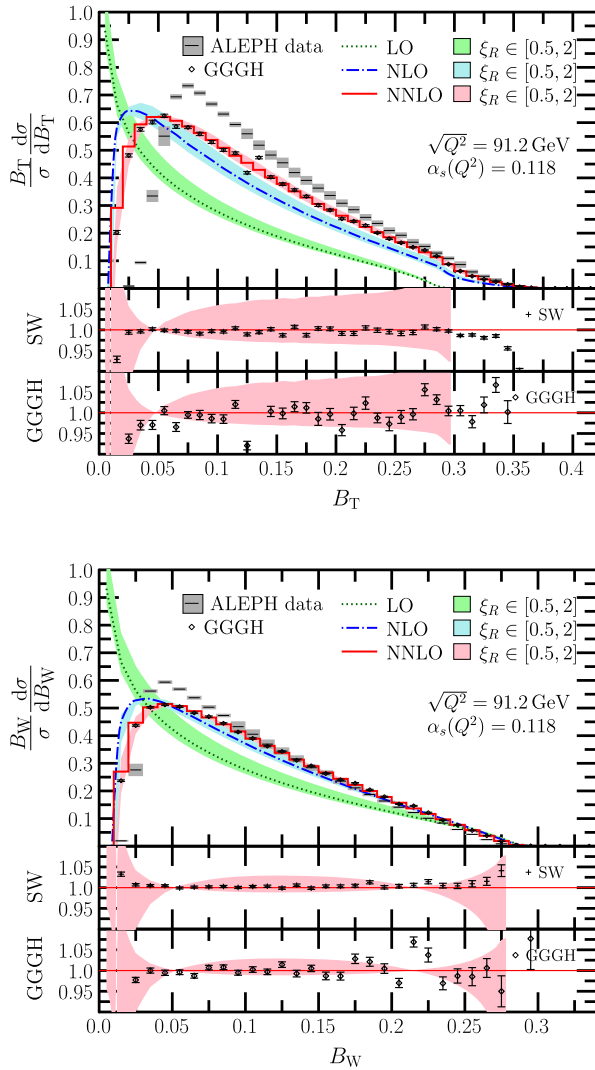
FIG. 2. Same as Fig. 1 for total ( B_T ) and wide ( B_W ) jet broadening.
