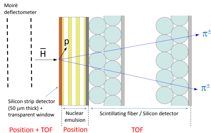
Figure 7. A design of the hybrid \bar{\text{H}} detector.
