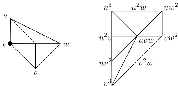
Figure 1. Polyhedron for dP_1 and its dual with corresponding monomials (in the patch e = 1 ). The toric zero section \hat{c}_0 is indicated by the dot.
