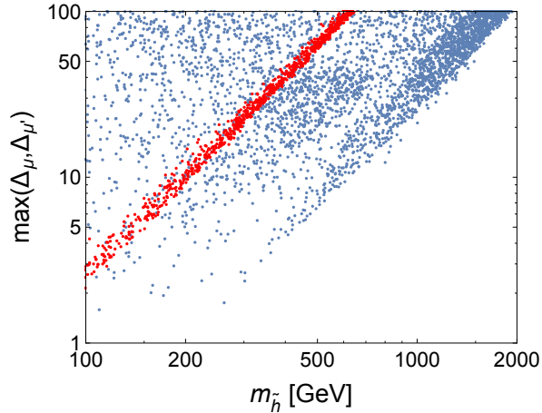
FIG. 2. The maximum \Delta_{\mu,\mu'} contribution to the fine tuning measure plotted against the Higgsino mass for varying \mu' (blue) and \mu' = 0 (red).
