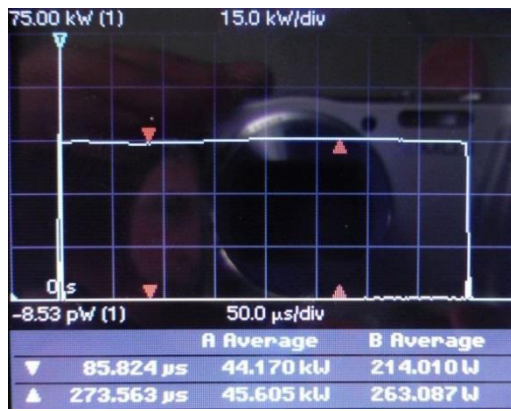
Figure 4: Undisturbed 0.4 ms long 45 kW RF pulse.
