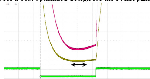
Figure 13: Vertical zoom of Fig. 12 (200 \mu s/div).
