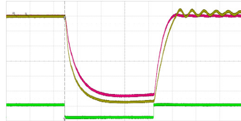
Figure 12: Modulator voltage and current (200 \mu s/div).
