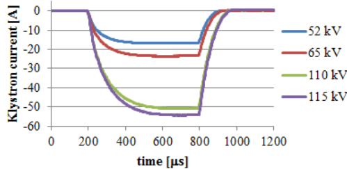
Figure 9: Klystron current measured in the oil tank.
