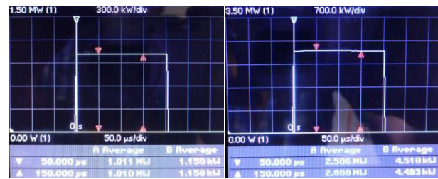
Figure 11: 1.0 and 2.5 MW klystron power (50 \mu s/div).
