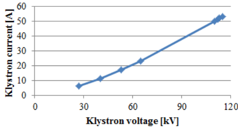
Figure 8: Klystron current vs. klystron voltage.
