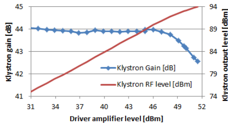
Figure 10: Driver level and klystron output power level.
