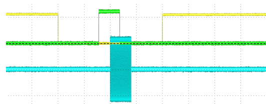
Figure 2: Amplifier test pulse pattern (0.5 ms/div).
