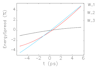
Figure 3: Longitudinal phase space at 3 positions before the bunch compressor, showing linearization of the curvature introduced by the RF curvative. Location where each phase space plot was generated is shown in Fig. 1.
