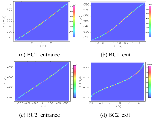
Figure 6: Longitudinal phase space evolution, through the two bunch compressors using Harmonic Linearization.
