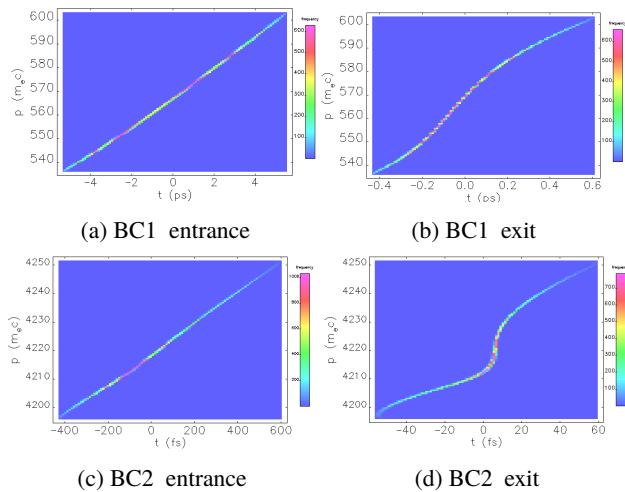
Figure 4: Longitudinal phase space evolution through two bunch compressors using Phase Modulation Linearization.
