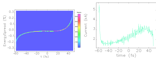
(a) Longitudinal phase space (b) Current profile
