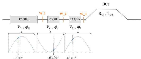
Figure 1: Layout of an x-band FEL accelerator design, up to end of first bunch compressor, which employs Phase Modulation Linearization. Included are markers showing location of longitudinal phase space plots in Fig. 3.
