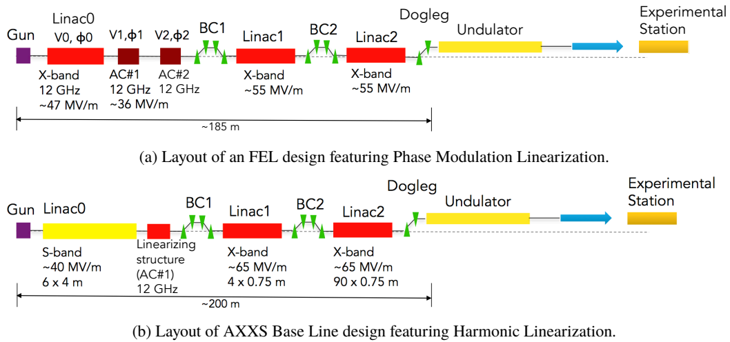
Figure 2: Two FEL design layouts each employing different techniques to linearize the longitudinal phase space.
