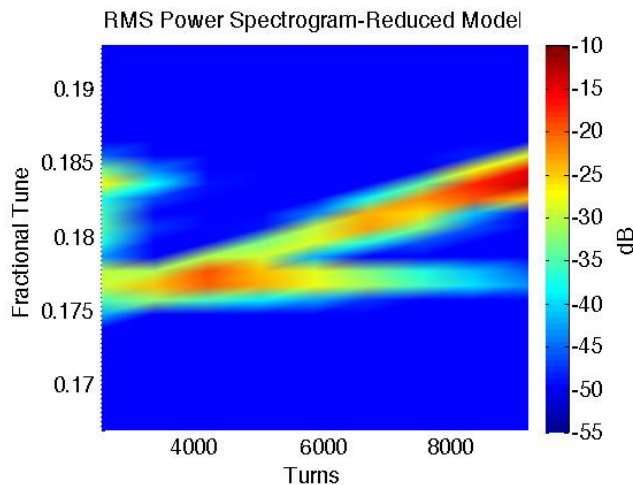
Figure 2: Beam motion spectrogram response for the reduced beam model (same excitation as Figure 1). Comparing with the physical measurement we see very close agreement between the oscillation frequencies and the amplitudes of the excited motion.
