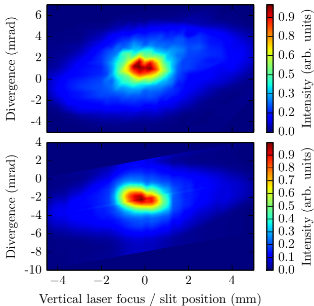
Figure 3: Vertical transverse phase space of the 3 MeV H^- beam measured by the laserwire (top) and conventional slit and grid (bottom) methods.
