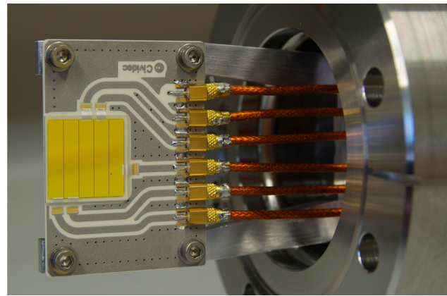
Figure 2: Photo of the “CIVIDEC” five strip diamond detector.
