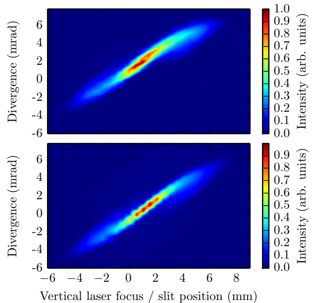
Figure 4: Vertical transverse phase space of the 12 MeV H^- beam measured by the laserwire (top) and conventional slit and grid (bottom) methods.
