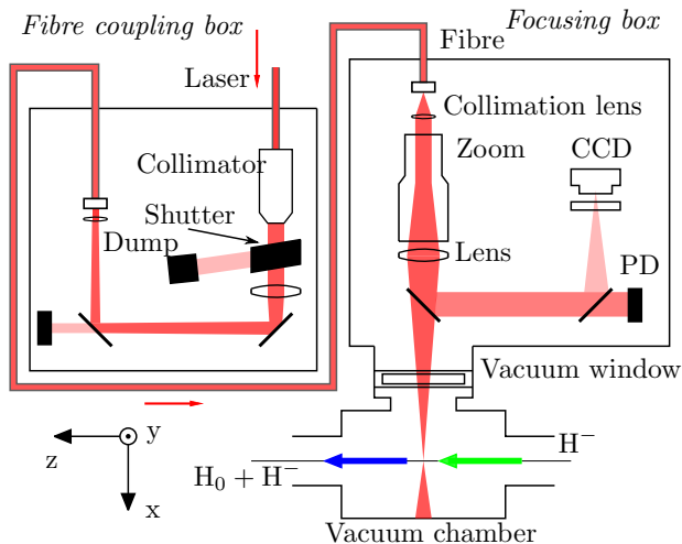
Figure 1: Schematic diagram of the laser delivery system.
