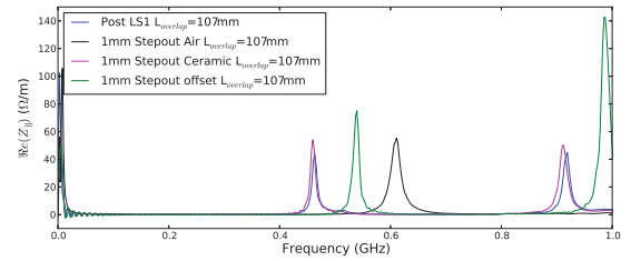
Figure 3: Real component of the longitudinal beam coupling impedance of an MKI with different longitudinal beam screen arrangements. The HV deflector is not included in this model.
