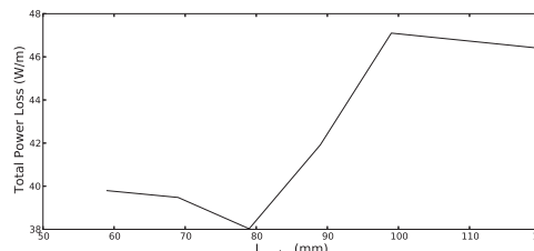
Figure 6: Power lost per metre for a number of overlap lengths, calculated assuming nominal LHC parameters using resonant wire measurements.
