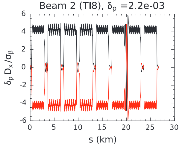
Figure 2: Worst-case off-momentum trajectory in the LHC for beam 2 with a momentum cut of \Delta p/p = \pm 0.22\% in TI 8.
