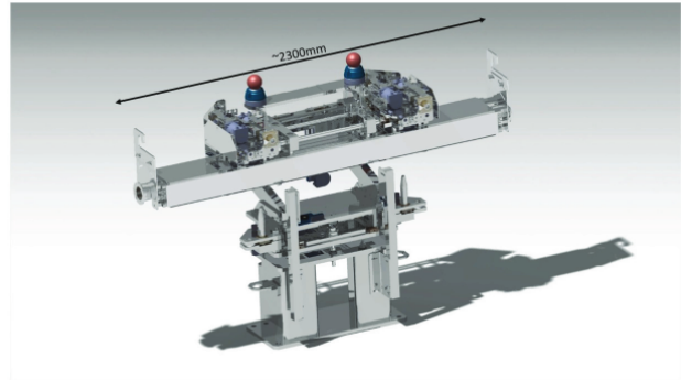
Figure 1: First version of 3D design of LIU transfer line collimator.
