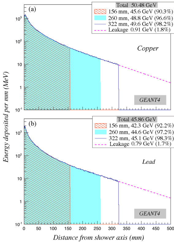
Fig. 24. Radial profiles for 60 GeV pions developing showers in the RD52 copper (a) or lead (b) based fiber calorimeters. Results from GEANT4 Monte Carlo simulations.
