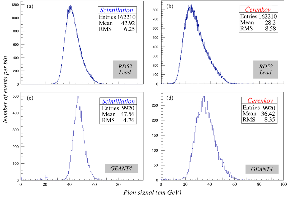
Fig. 18. The response functions for 60 GeV pions in the lead based RD52 calorimeter. Shown are the experimental data measured for the scintillation (a) and Cerenkov (b) signals, as well as the simulated response functions for these two types of signals (c and d).
