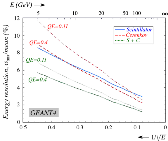
Fig. 17. The predicted effect of an increase in the Cherenkov light yield on the em energy resolution of the copper calorimeter. See text for details.
