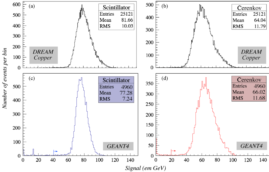
Fig. 19. The response functions for 100 GeV pions in the copper based DREAM calorimeter. Shown are the experimental data measured for the scintillation (a) and Cerenkov (b) signals [8], as well as the simulated response functions for these two types of signals (c and d).
