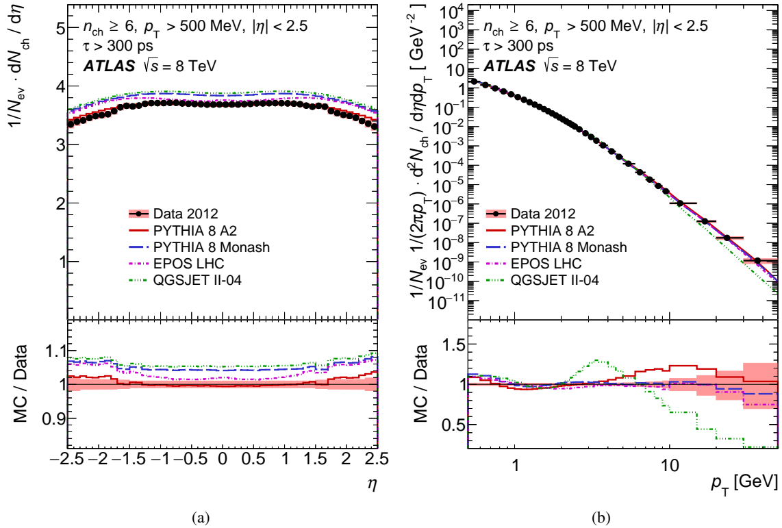
Figure 6: Distributions of primary charged particles in events for which n_{\text{ch}} \geq 6 , p_{\text{T}} > 500 MeV and |\eta| < 2.5 as a function of (a) pseudorapidity, \eta , and (b) transverse momentum, p_{\text{T}} . The data, represented by dots, are compared to various particle-level MC predictions, which are shown by curves. The shaded areas around the data points represent the total statistical and systematic uncertainties added in quadrature.
