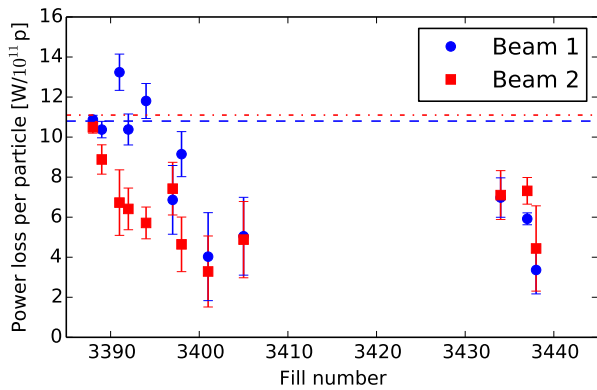
Figure 3: Evolution of the maximum power loss per particle at 450 GeV during the scrubbing run (25 ns beams) in 2012 for Beam 1 (blue circles) and for Beam 2 (red squares). The dashed lines represent the scrubbing level achieved in 2011 for both beams. Error-bars are calculated from the noise of the bunch-by-bunch phase measurements.
