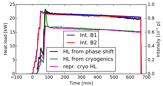
Figure 2: Total beam power loss found from the phase shift (black line) and the heat load measured by the cryogenic system (green line) [9, 10], for a fill with 25 ns beams accelerated to 4 TeV in December 2012. An estimation to the cryogenic heat load (magenta line) was calculated from the phase shift measurements as described in the text (scale factor 0.76 to fit the part at 4 TeV).
