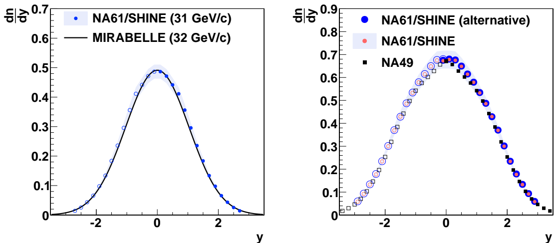
Figure 6.22: Comparisons of the rapidity distribution of the \pi^- mesons produced in inelastic p+p interactions. Left : The NA61/SHINE results at 31 GeV/c (blue points) are compared with the MIRABELLE measurement (parametrised by the black line) at 32 GeV/c. The shaded band shows the NA61/SHINE systematic uncertainty. Right : Rapidity distribution of the \pi^- mesons produced in inelastic p+p interactions at 158 GeV/c. The large blue points show the results obtained with an alternative method: without vertex fit requirement and rejection of events with a single very high momentum positively charged track. The results of NA61/SHINE (red dots) are compared with the NA49 measurements [25] (black squares). The open symbols show points reflected with respect to mid-rapidity. A single NA61/SHINE point measured at y < 0 is also shown for comparison. The shaded band shows the NA61/SHINE systematic uncertainty.
