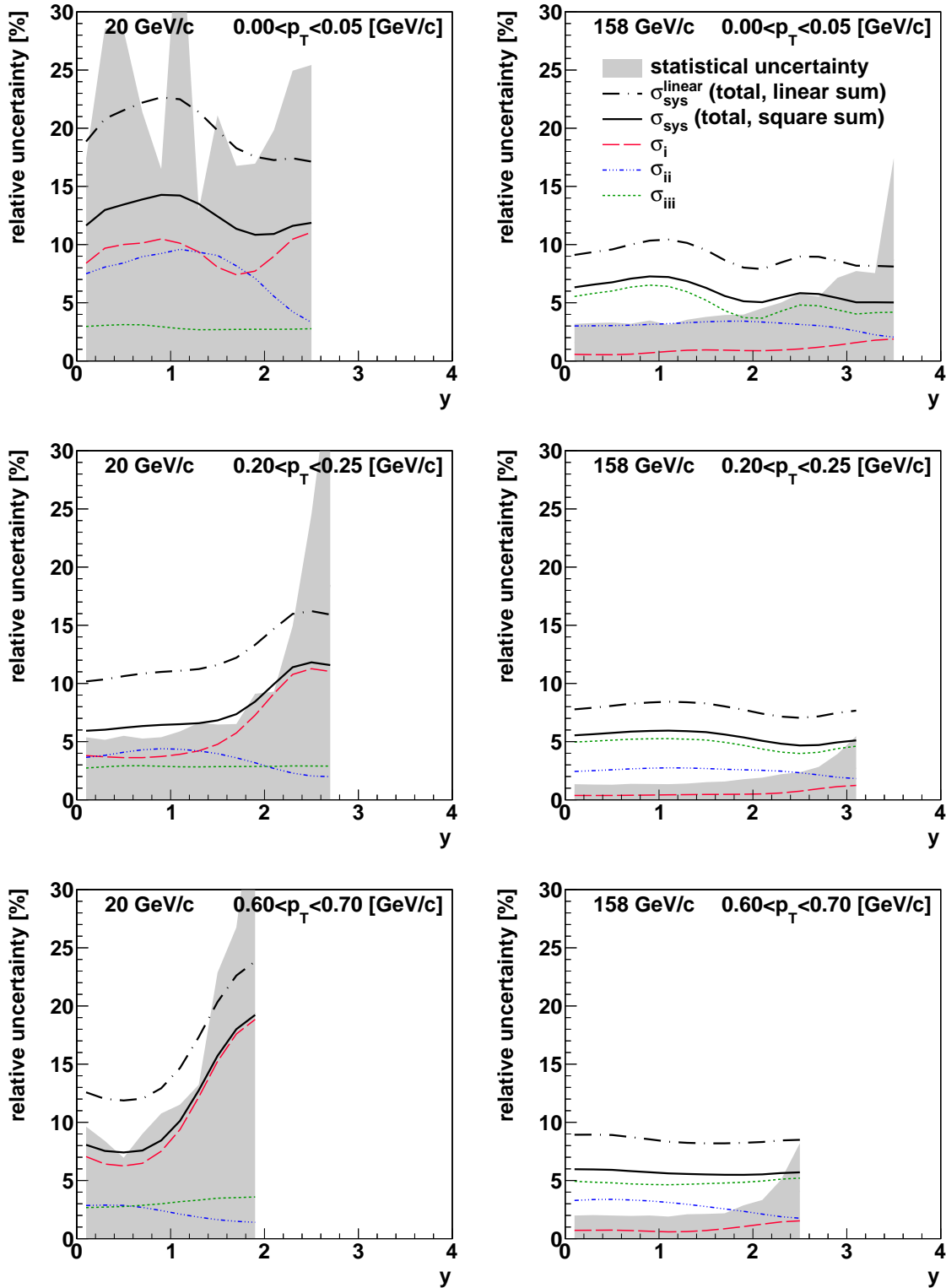
Figure 6.17: Statistical and systematic uncertainties in selected p_T bins for 20 ( left ) and 158 GeV/c ( right ) p+p data. The shaded band shows the statistical uncertainty; at 20 GeV/c the uncertainty exceeds the vertical scale on the plot in several bins. The coloured thin lines show the contributions to the systematic uncertainty listed in Sect. 6.5.2. The thick black lines show the total systematic uncertainty, which was calculated by adding the contributions in quadrature (continuous line) or linearly (dashed/dotted line).
