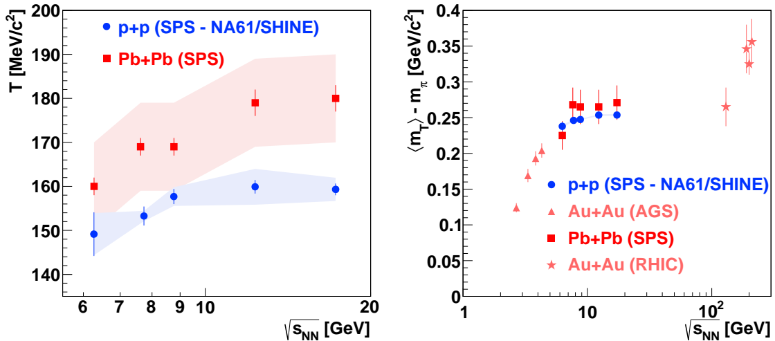
Figure 7.5: Left : Inverse slope parameter T of the transverse mass spectra at mid-rapidity ( 0 < y < 0.2 ) plotted against the collision energy per nucleon. The parameter T was fitted in the range 0.2 < (m_T - m_\pi) < 0.7 \text{ GeV}/c^2 . The systematic uncertainty is shown with faded bands. As for the two lowest energy points for Pb+Pb, the systematic uncertainty was not given in [9], it is assumed to be the same as for the higher energies [8]. Right : The mean transverse mass \langle m_T \rangle at mid-rapidity ( 0 < y < 0.2 ) versus the collision energy. The results on inelastic p+p interactions are compared with the corresponding data on central Pb+Pb and Au+Au collisions.
