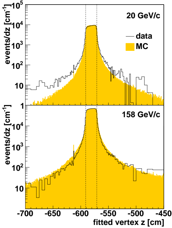
Figure 4.6: Distribution of fitted vertex z coordinate for p+p interactions at 20 (top) and 158 GeV/c (bottom) in the target vicinity ( -591 < z_{\text{target}} < -571 cm, marked with vertical dashed lines). The solid line shows the distribution of interactions with the hydrogen target in the data. The filled area shows the distribution for the reconstructed Monte Carlo simulation. This distribution was normalised to the total integral of the data plot.
