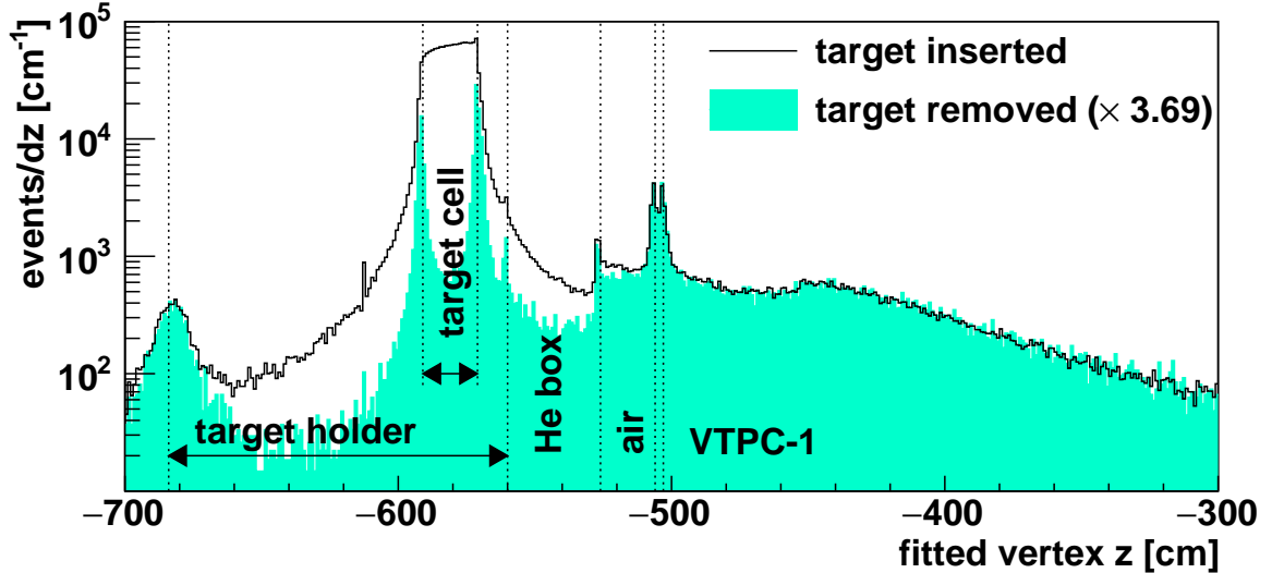
Figure 3.12: Distribution of the fitted vertex z coordinate for interactions of proton beam at 40 GeV/ c with target inserted and removed. Peaks in the histogram reflect the distribution of the material along the beam line: liquid hydrogen, walls, vacuum, helium, and the TPC working gas.
