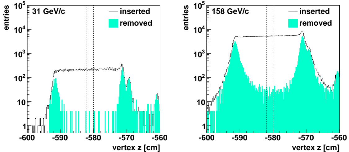
Figure 5.7: Distributions of the fitted vertex z coordinate for the target inserted and removed in events taken with an unbiased beam trigger at 31 GeV/c ( left ) and 158 GeV/c ( right ). For the best resolution, only events with at least 7 tracks were selected. The target removed distribution was normalised to the vertex distribution far away from the target cell, as described in Sect. 6.4.1. The vertical dashed lines show the z range used to calculate the interaction rates shown in Fig. 5.8.
