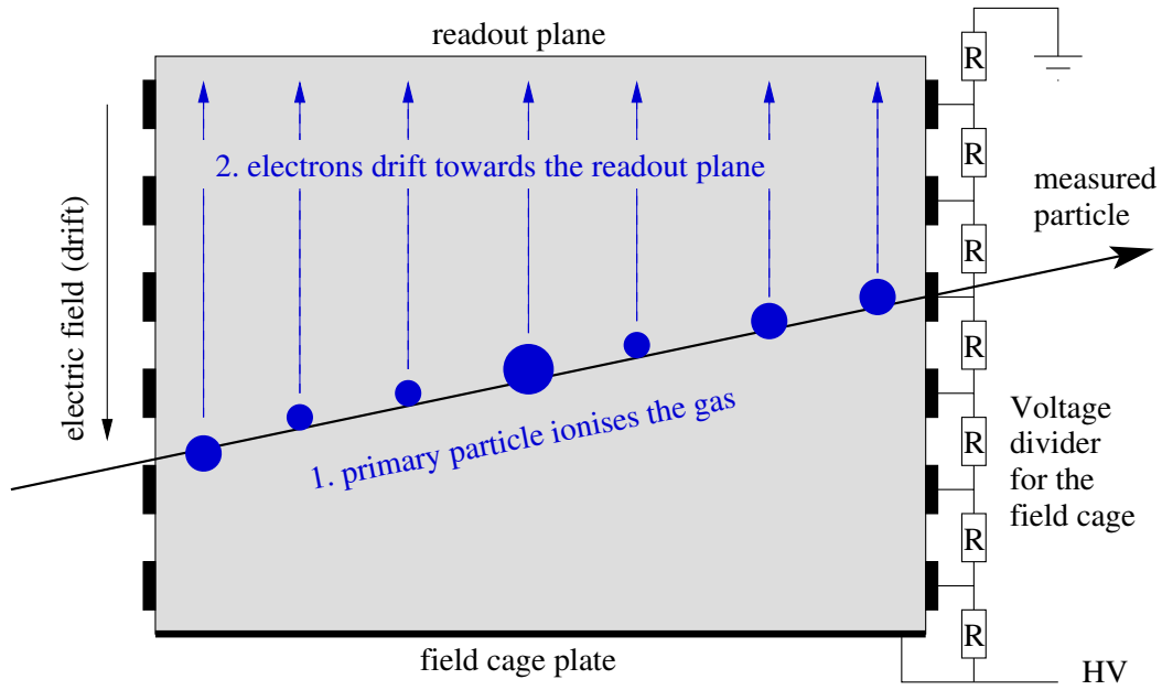
Figure 3.1: A schematic of a TPC. The active volume ( grey ) is enclosed in a field cage, consisting of an anode ( top ) and a cathode ( bottom ) plate, and a number of strips on the sides with gradually changing voltage. Electrons resulting from ionisation induced by the primary particle drift in presence of the electric field.
