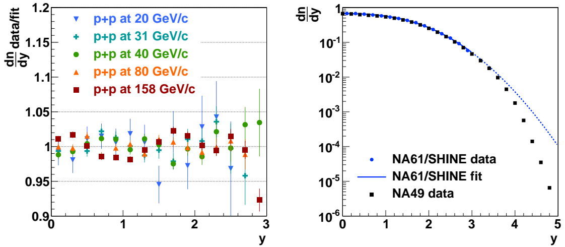
Figure B.4: Comparison of parametrisation of the rapidity distribution (Eq. (B.9)) and the measured data points. Left : Data divided by the parametrisation at five beam momenta. Right : comparison of the data on p+p interactions at 158 GeV/c measured by NA61/SHINE and NA49 [25] with the fitted parametrisation (solid line) and extrapolated parametrisation (dashed line).
