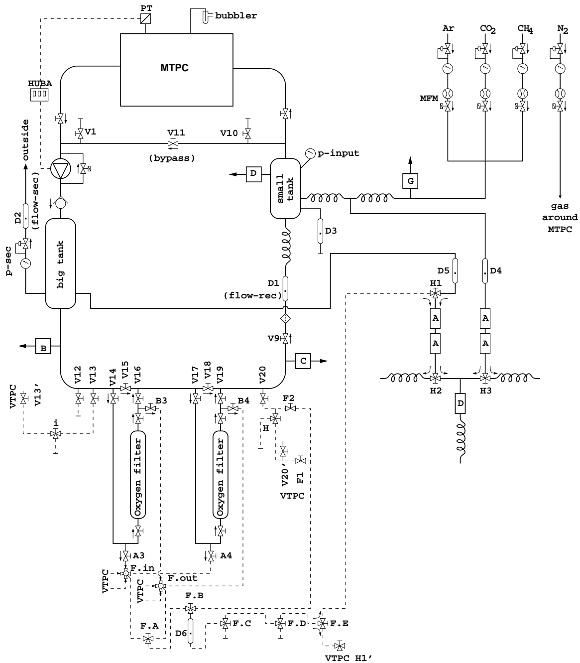
Figure 3.7: A schematic of the gas system of one of the MTPCs. The schematic for VTPCs is almost identical. The symbols used are explained in Fig. 3.8. The main parts are drawn with bold lines; the dashed lines show connections not used in the regular operation modes. The gas mixing system is shown in the upper right corner. The fresh gas enters the small buffer tank and then the TPC. A compressor pumps the gas out of the TPC and circulates it through the oxygen filter. The oxygen and water content in the gas can be monitored in points labelled B, C, D and G. The drift velocity and the gas amplification can be measured in fresh gas and in gas coming from the TPC in the monitors drawn on the right side, labelled D and A, respectively.
