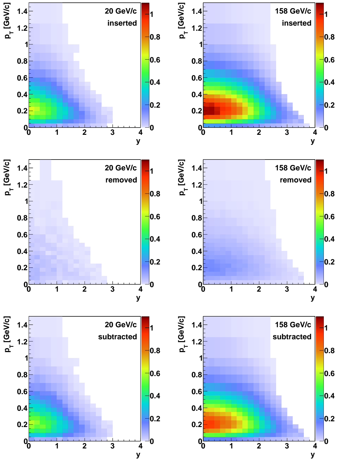
Figure 6.11: Negatively charged hadron spectra after event and track selection for target inserted n_I[h^-]/(1 - \varepsilon) (top), removed n_R[h^-]\varepsilon/(1 - \varepsilon) (middle) and their difference (bottom) n_T[h^-] , normalised as in Eq. (6.4), for 20 (left) and 158 GeV/c (right).
