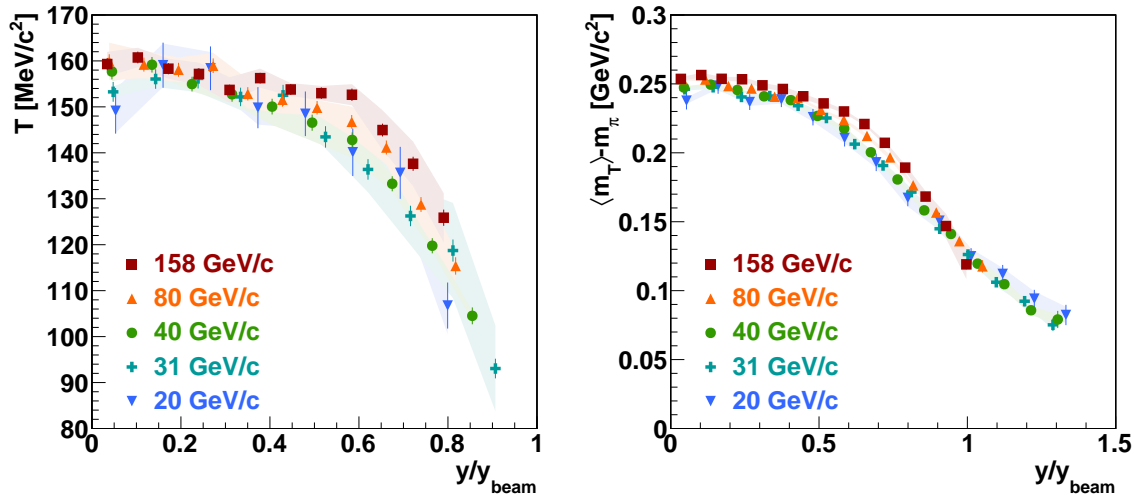
Figure 7.3: Left: The inverse slope parameter T of the transverse mass spectra as a function of rapidity divided by the projectile rapidity y_{\text{beam}} ( = 1.877, 2.094, 2.223, 2.569 and 2.909 at 20, 31, 40, 80 and 158 GeV/c, respectively). The fit range is 0.2 < (m_T - m_\pi) < 0.7 \text{ GeV}/c^2 . Right: The mean transverse mass \langle m_T \rangle as a function of rapidity divided by the projectile rapidity. The results in both panels refer to the \pi^- mesons produced in inelastic p+p interactions at 20, 31, 40, 80 and 158 GeV/c.
