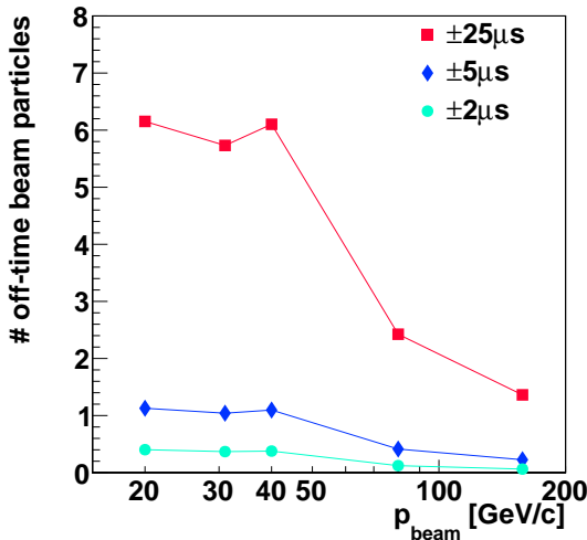
Figure 5.3: The average number of the off-time beam particles per event within \pm 2 , \pm 5 and \pm 25 \mu s around the trigger particle, at five beam momenta.
