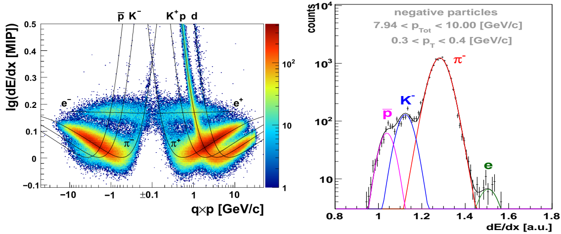
Figure 3.4: Particle identification in NA61/SHINE Time Projection Chambers. Left : logarithm of the measured energy loss in TPCs as a function of momentum times electric charge of the measured particle. Each entry on the histogram corresponds to a single particle. Theoretical Bethe curves are drawn over the measured data. Right : the dE/dx distribution in the selected momentum range of 7.94–10.00 GeV/c for the transverse momentum range of 0.3–0.4 GeV/c. The fitted lines indicate contributions of various particle types. Figures obtained from Ref. [48].
