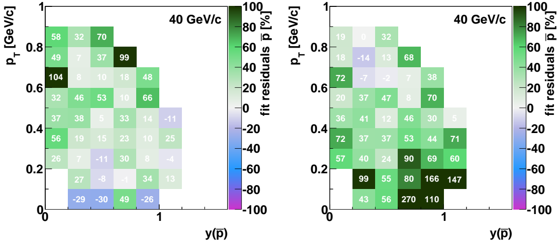
Figure 4.4: Residuals of the function a[\bar{p}] (Eq. (4.6)) and the data ratio r[\bar{p}] (Eq. (4.4)) using the best fit of the D_{\bar{p}} parameter ( left , see Fig. 4.3), and D_{\bar{p}} calculated from Eq. (4.7) ( right ) at 40 GeV/c. The plotted residuals are defined as \text{residuals} = (a[\bar{p}]/r[\bar{p}] - 1) \cdot 100\% .
