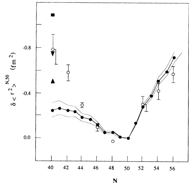
FIG. 8. Comparison between experimental \delta\langle r^2 \rangle values (solid circles connected by a solid line) and the results from the HF calculations using force SKa, for Sr isotopes in the region of predicted spherical shapes. The theoretical \delta\langle r^2 \rangle values are corrected for deformation using experimental B(E2) values as described in the text. For N=40 , the results of HF calculations with different interactions are shown for the case when a rigidly deformed nuclear charge distribution with \beta=0.42 is assumed. The quadrangle represents the result for force SKa; the triangle that for force S III and the inverted triangle that for force S VI.
