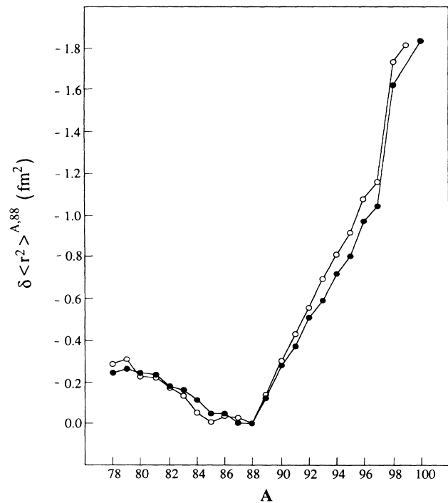
FIG. 5. Changes in mean square charge radii of Sr isotopes (solid circles). The data points are connected by a solid line to guide the eye. The results for Rb (Ref. 12) are added for comparison.
