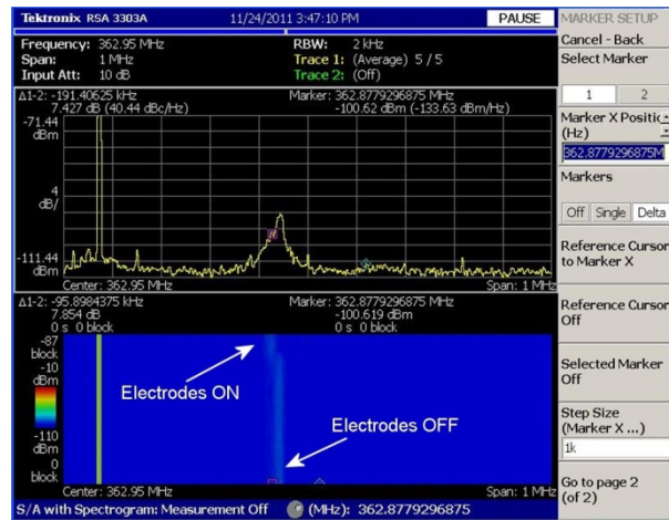
Figure 2: horizontal tune shift measured with 550 mA of positron beam. The image is taken from the spectrum analyser connected to one button pickup.
