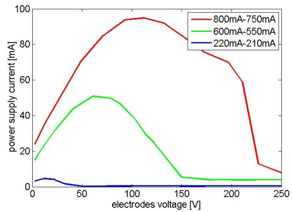
Figure 7: current supplied by the dc voltage generator as a function of the applied voltage and beam current.
