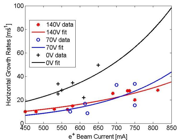
Figure 5: growth rates of the horizontal instability.
