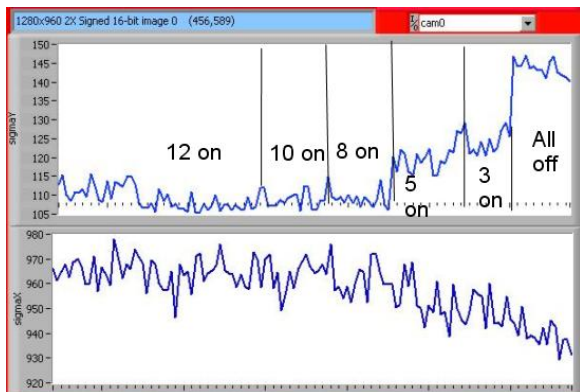
Figure 4: Beam dimension (in \mu\text{m} ) at the SLM turning off, progressively, all electrodes.
