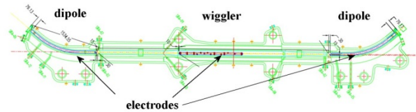
Figure 1: mechanical drawing of an arc with the electrodes.
