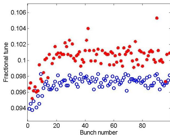
Figure 3: horizontal fractional tune as a function of bunch number (blue curve: electrodes ON, I_B=550\text{mA} ; red curve: electrodes OFF, I_B=600\text{mA} ).
