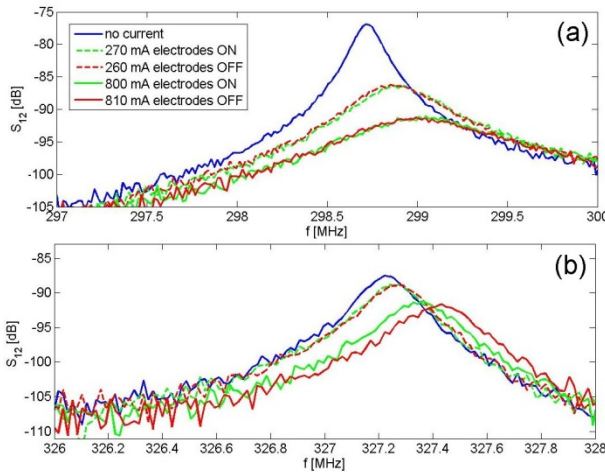
Figure 6: transmission coefficient between two button pickup in the arc chamber for two different resonant modes.
