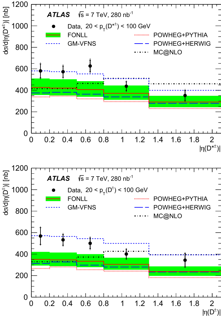
Fig. 6. Differential cross sections for D^{*\pm} (top) and D^\pm (bottom) mesons with 20 < p_T(D) < 100 \text{ GeV} as a function of |\eta| for data (points) compared to the NLO QCD calculations of FONLL, POWHEG + PYTHIA, POWHEG + HERWIG, MC@NLO and GM-VFNS (histograms). The data points are drawn in the bin centres. The inner error bars show the statistical uncertainties and the outer error bars show the statistical and systematic uncertainties added in quadrature. Uncertainties linked with the luminosity measurement (3.5%) and branching fractions (1.5% and 2.1% for D^{*\pm} and D^\pm , respectively) are not included in the shown systematic uncertainties. The bands show the estimated theoretical uncertainty of the FONLL calculation.
