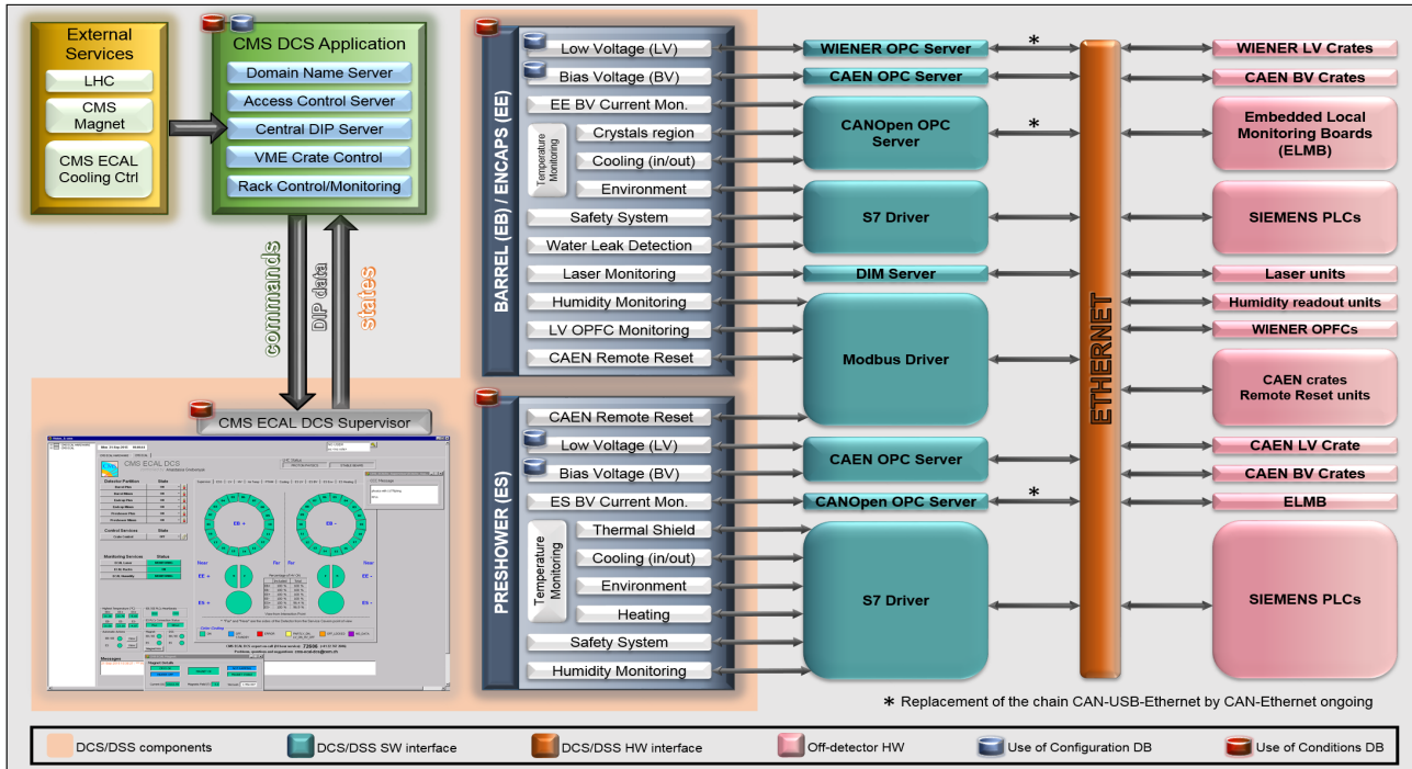
Figure 1: Simplified block diagram of the CMS ECAL Control and Safety Systems
