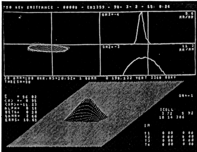
Fig. 6 RFQ2 output emittance
