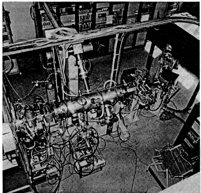
Fig. 4 RFQ2 in its experimental area
