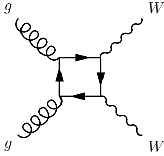
Figure 4.2: W^+W^- production diagram from gluon-gluon initial state.
