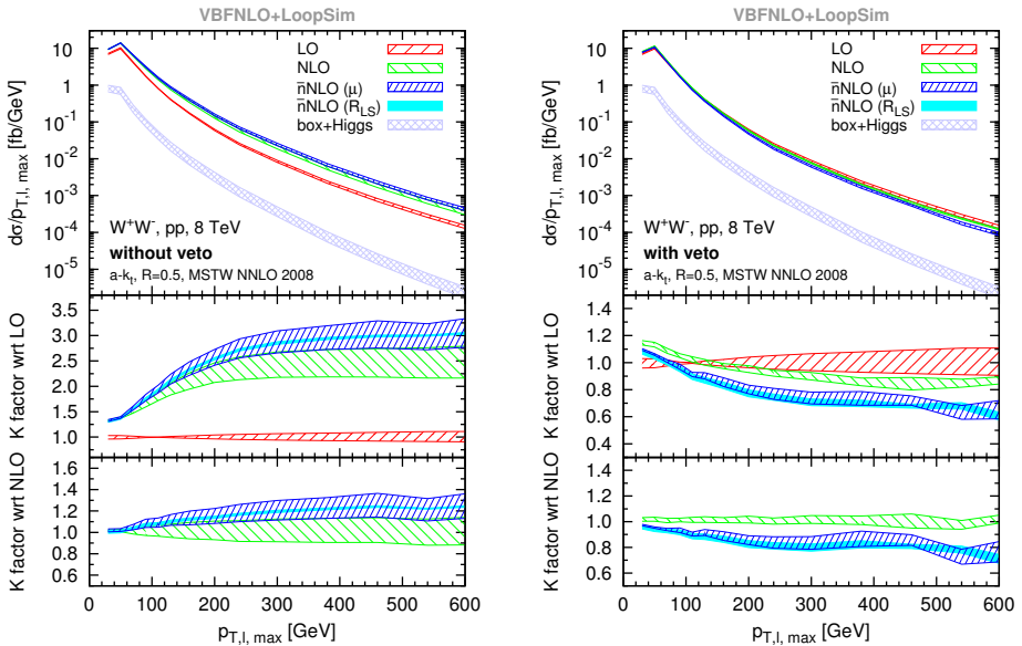
Fig. 2. Differential cross sections and K -factors for the p_T of the hardest lepton at \sqrt{s} = 8 \text{ TeV} without (left) and with jet veto (right). Bands are defined as in Fig. 1. We include the channels e^+\nu_e e^-\bar{\nu}_e , \mu^+\nu_\mu \mu^-\bar{\nu}_\mu , e^+\nu_e \mu^-\bar{\nu}_\mu and \mu^+\nu_\mu e^-\bar{\nu}_e . The contribution from the gluon-fusion box and Higgs diagrams is included in the NLO and \bar{n} NLO curves. The left panels correspond to the inclusive sample, while the results shown in the right panel were obtained with vetoing events containing jets which fulfill the criteria p_{T,\text{jet}} > 30 \text{ GeV} and |\eta_{\text{jet}}| < 4.7 .
