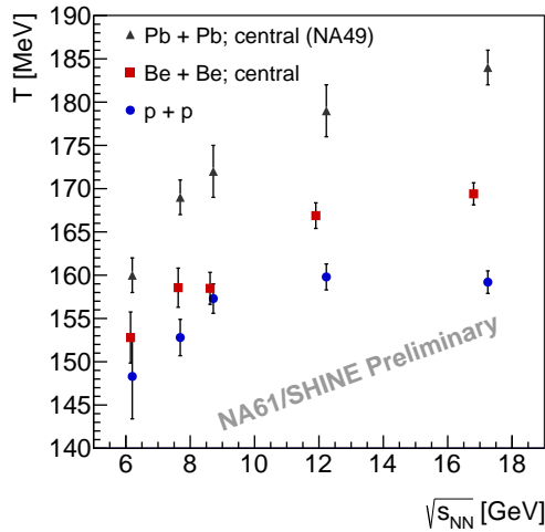
Figure 11: Inverse slope parameter T obtained from \pi^- transverse mass distributions at mid-rapidity for p+p [2] and central {}^7\text{Be}+{}^9\text{Be} and \text{Pb}+\text{Pb} [31] collisions. The high inverse slope parameter in \text{Pb}+\text{Pb} interactions is due to radial flow. The values of T for {}^7\text{Be}+{}^9\text{Be} are between those of p+p and \text{Pb}+\text{Pb} collisions and can be interpreted as possible evidence of transverse collective flow in central {}^7\text{Be}+{}^9\text{Be} interactions. Note: the fitted inverse slope parameter T in A+A collisions is sensitive to the fit range and the location of the rapidity bin.
