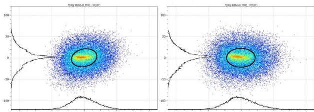
Figure 7: Expected (left) and reconstructed (right) beam distribution in the longitudinal phase space at RFQ output.
