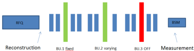
Figure 5: Longitudinal emittance reconstruction setup (quads in blue, bunchers in green and red)
