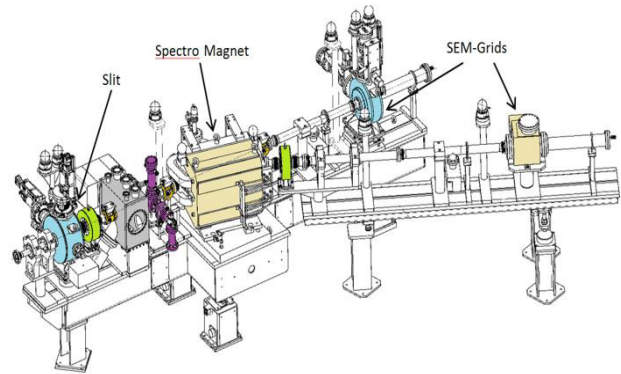
Figure 1: The low energy diagnostic bench.
