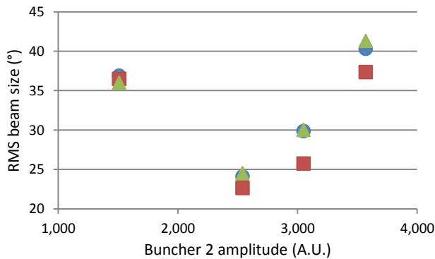
Figure 6: Predicted (red), measured (blue) and reconstructed (green) longitudinal rms beam sizes.
