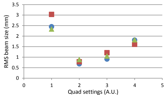
Figure 4b: Predicted (red), measured (blue) and reconstructed (green) vertical rms beam sizes for different quadrupole settings.
