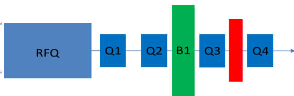
Figure 3: Layout of the first MEBT section (quads in blue, buncher in green and wire-scanner in red).
