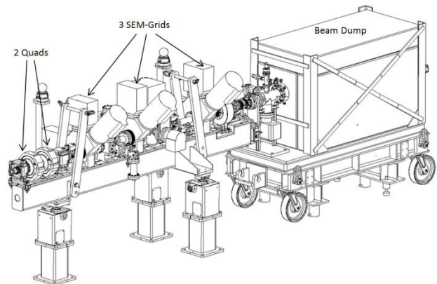
Figure 2: The high energy diagnostic bench.
