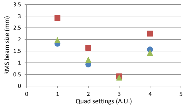
Figure 4a: Predicted (red), measured (blue) and reconstructed (green) horizontal rms beam sizes for different quadrupole settings.
