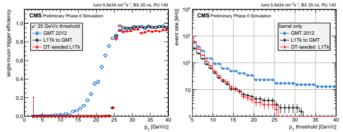
Figure 2: Efficiency of a single muon trigger with p_T threshold at 25 GeV/c for muons ionising the gas mixture in the DT chambers, as a function of the generated muon p_T (left) and expected background rate as a function of the threshold for single muon trigger, at the average pile-up of 140, with 25 ns bunch separation and 0.75 fill factor (right). Generated muons with flat p_T distribution in the 2–160 GeV/c range are superimposed to minimum-bias background at the average pile-up of 140 with 25 ns bunch separation. The performance of the DT-seeded algorithm (red) is compared to those of the Run 1 Global Muon Trigger (blue) and inside-out muon track trigger (black), only for candidates built from signals collected in the barrel.
