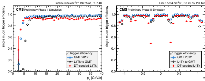
Figure 1: Trigger efficiency for muons ionising the gas mixture in the DT chambers, as a function of the generated muon p_T (left) and \eta (right). Generated muons with flat p_T distribution in the 2–160 GeV/c range are superimposed to minimum-bias background at the average pile-up of 140 with 25 ns bunch separation. The performance of the DT-seeded algorithm (red) is compared to those of the Run 1 Global Muon Trigger (blue) and inside-out muon track trigger (black), only for candidates built from signals collected in the barrel. The track preselection of the inside-out muon track trigger can still be tuned up to improve the efficiency at low p_T . Gaps in \eta are due to the geometry of the DT system: they are more significant for the DT-seeded algorithm as it does not make use of all four stations and seeding does not combine different wheels.
