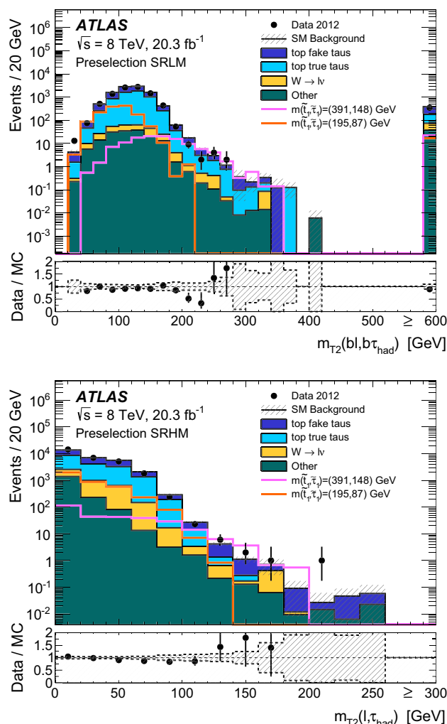
Fig. 4 Top Distribution of the transverse mass constructed from the b -jet plus lepton and b -jet plus \tau_{had} , m_{T2}(b\ell, b\tau_{had}) , for events passing the lepton–hadron preselection requirements with the additional requirement of a second b -tagged jet. Bottom Distribution of the transverse mass constructed from the momenta of the light lepton and the hadronically decaying tau, m_{T2}(\ell, \tau_{had}) , for events passing the lepton–hadron preselection requirements. The contributions from all SM backgrounds are shown as a histogram stack; the bands represent the total uncertainty. The overflow bin in the m_{T2}(b\ell, b\tau_{had}) plot is filled with the events that have no (b\ell, b\tau_{had}) pairing satisfying m(b\ell) < m_t and m(b\tau_{had}) < m_t . The distributions expected for two signal models are also shown
