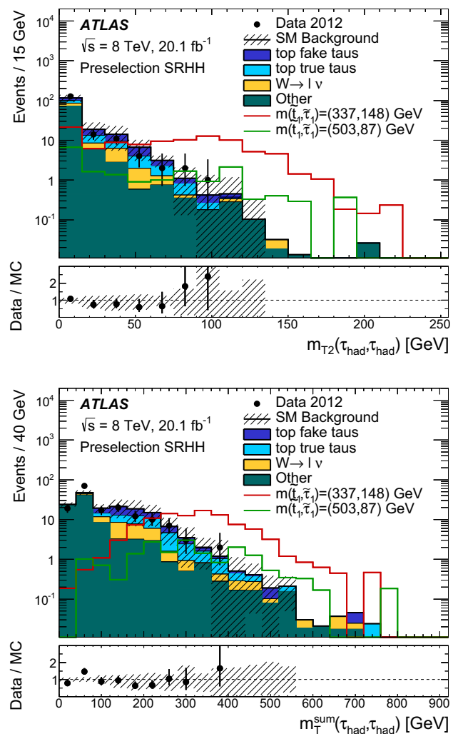
Fig. 2 Top Distribution of the transverse mass constructed from the two \tau_{\text{had}} , m_{T2}(\tau_{\text{had}}, \tau_{\text{had}}) , for events passing the hadron–hadron preselection requirements. Bottom Distribution of the sum of the transverse mass of each \tau_{\text{had}} candidate and the missing transverse momentum, m_T^{\text{sum}}(\tau_{\text{had}}, \tau_{\text{had}}) , for events passing the hadron–hadron preselection requirements. The contributions from all SM backgrounds are shown as a histogram stack; the bands represent the total uncertainty. The distributions expected for two signal models are also shown
