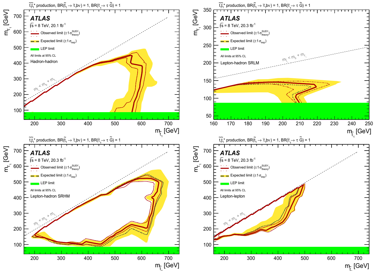
Fig. 10 Observed and expected exclusion contours at 95 % CL in the (\tilde{t}_1, \tilde{\tau}_1) mass plane from the hadron–hadron ( top left ), the lepton–hadron low-mass ( top right ), the lepton–hadron high-mass ( bottom left ) and the lepton–lepton selections of Ref. [50] ( bottom right ). The dashed and solid lines show the 95 % CL expected and observed limits, respectively, including all uncertainties except for the theoretical signal cross-section
