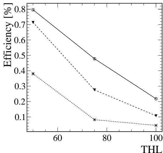
Figure 13. Overall hit efficiency in irradiated assembly W20_D6 with 200 \mu\text{m} thick n -on- p sensor as function of the THL value for different bias voltages (stars: -100 V, triangles: -200 V, circles: -300 V). The assembly was irradiated to a fluence of 2.5 \times 10^{15} 1 \text{ MeV } n_{\text{eq}} \text{ cm}^{-2} . The lines are drawn to guide the eye.
