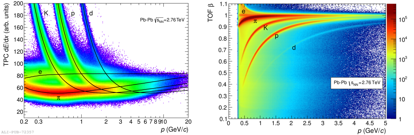
Figure 2.10: Particle identification for Pb–Pb collisions at \sqrt{s_{\text{NN}}} = 2.76 TeV for two systems in ALICE: the energy loss of the particles in the TPC (left panel) and the correlation \beta = v/c observed by TOF (right panel) versus the momentum.
