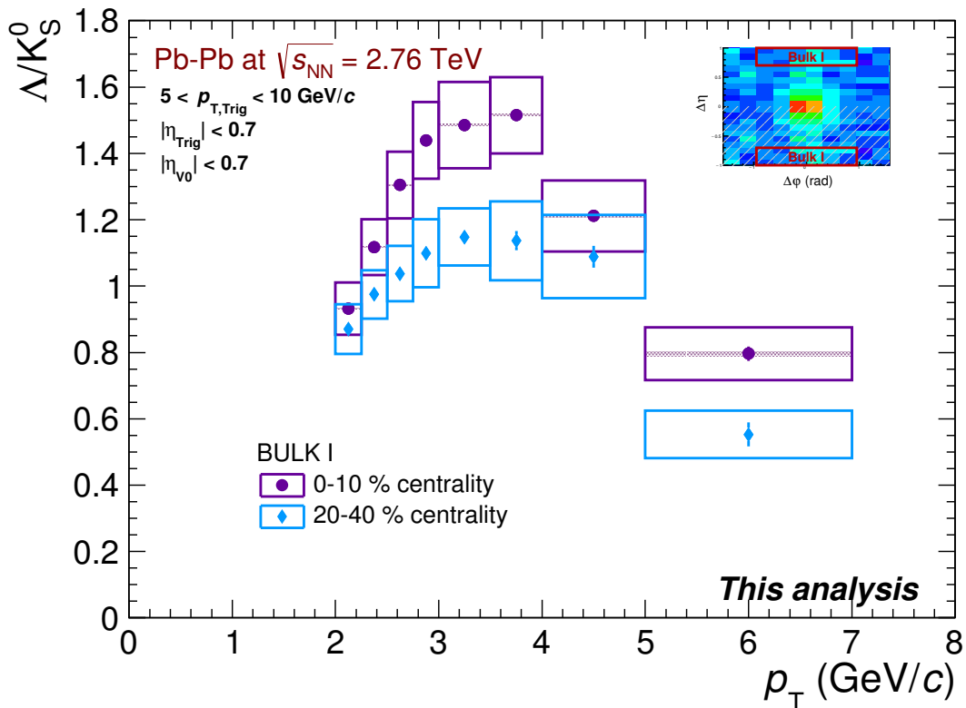
Figure 4.9: \Lambda/K_S^0 ratio obtained from the particles produced in the bulk I for the centrality intervals 0-10% and 20-40% in Pb-Pb collisions at \sqrt{s_{\text{NN}}} = 2.76 TeV for the 2011 run. The horizontal extension of the boxes represent the p_T -bin width. The markers are located at the middle value of the bin. The \bar{\Lambda} is not included in the per-trigger yield extraction. The empty (filled) boxes indicates the contributions of the uncorrelated (partially correlated) systematic uncertainties.
