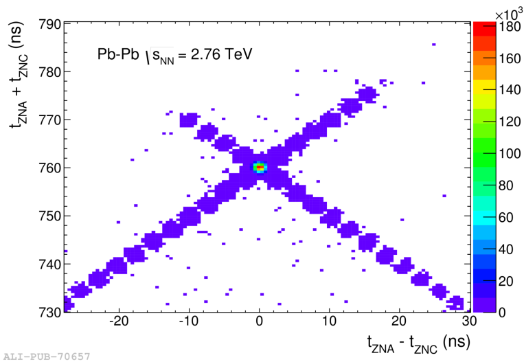
Figure 3.2: Correlation between the sum and the difference of the times recorded by the neutron ZDC detector on each side of the interaction region [132].
