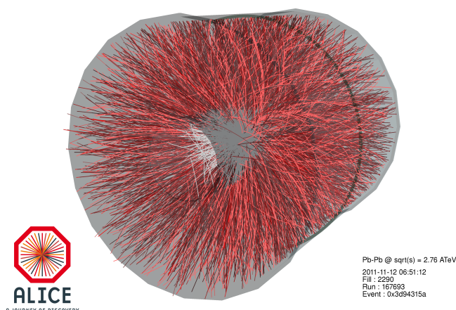
Figure 2.2: An event display of one Pb–Pb collision recorded with the ALICE detector in November 2010.
