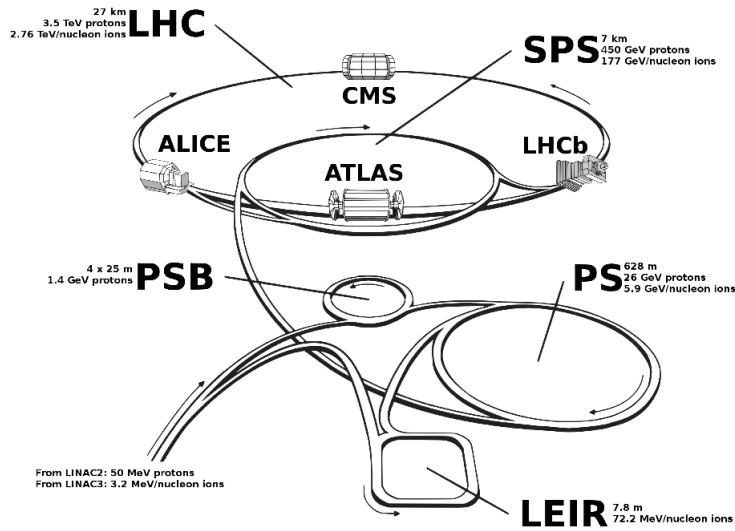
Figure 2.1: Large hadron collider scheme with the principal experiments [133].
