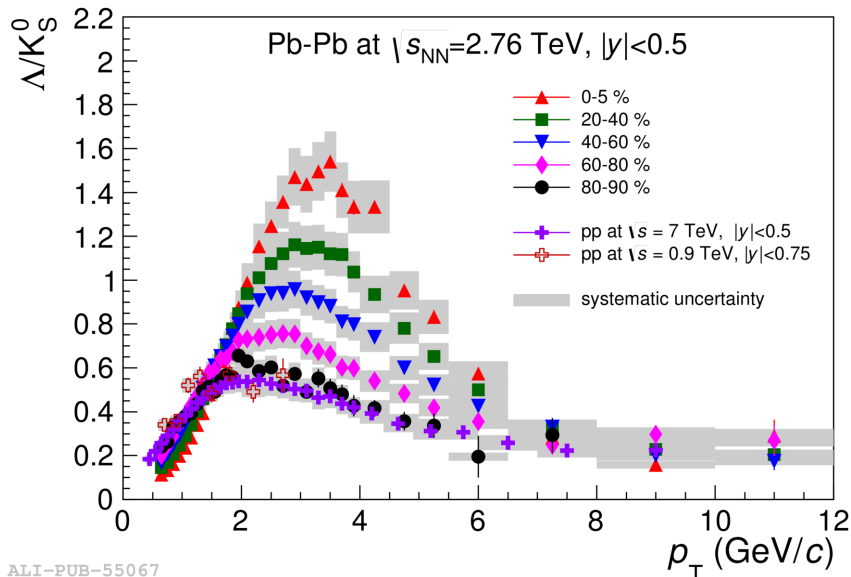
Figure 1.10: \Lambda/K_S^0 ratio measured by ALICE in Pb–Pb collision at \sqrt{s_{\text{NN}}} = 2.76 TeV for different centrality intervals [117]. Results from pp collisions are also plotted for comparison.
