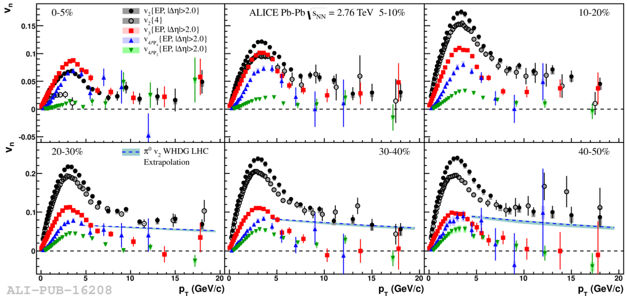
Figure 1.8: ALICE measurements of the elliptic flow and higher harmonics ( v_3 and v_4 ) for unidentified charged particles as a function of transverse momentum for various centrality classes [106].
