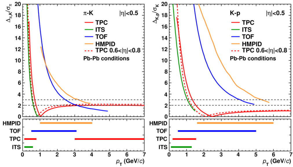
Figure 2.11: Separation power of hadron identification in the ITS, TPC, TOF, and HMPID as a function of the transverse momentum at midrapidity. The left panel shows the separation of pions and kaons, meanwhile the right panel corresponds to power separation of kaons and protons [132].
