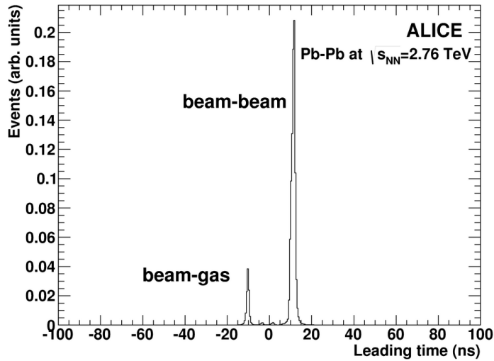
Figure 3.1: Time distribution of signals registered in the VZERO-A detector. The time arrival is measured with respect to the beam crossing time [155]. The beam-gas interactions are detected at earlier times than the beam-beam collisions.
