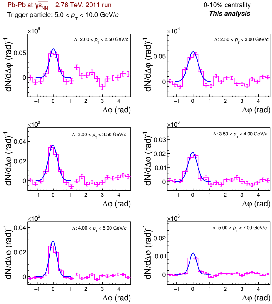
Figure E.2: h^\pm - \Lambda angular correlations in \Delta\varphi after subtraction of the elliptic flow. The results are presented for the 0-10% centrality class obtained with the 2011 Pb-Pb data. The Gaussian curve (in blue) describes the particle production related mostly to parton fragmentation.
