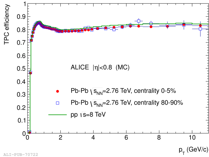
Figure 2.9: Tracking efficiency of charged primary particles reconstructed only in the TPC. The results are obtained for pp collisions and Pb–Pb collisions at LHC energies [132].
