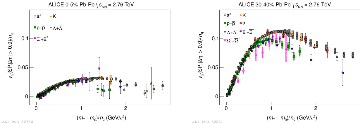
Figure 1.9: The (m_T - m_0)/n_q dependence of the quark-scaling elliptic flow ( v_2/n_q ) for identified hadrons for Pb–Pb collisions at \sqrt{s_{\text{NN}}} = 2.76 TeV in the centrality intervals 0-5% (left panel) and 30-40% (right panel) measured with ALICE [112].
