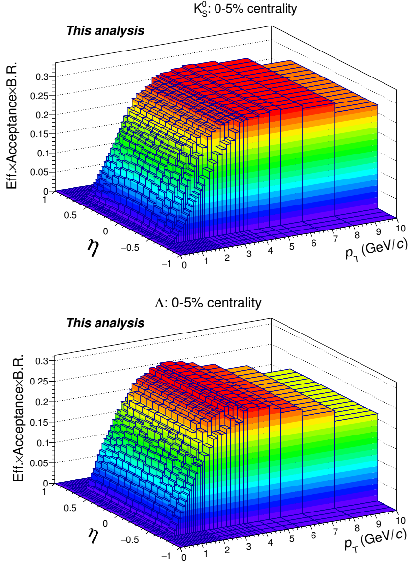
Figure 3.20: Efficiency \times Acceptance \times B.R. as function of pseudo-rapidity and transverse momentum of K_S^0 and \Lambda for the 2011 data taking period in the 0–5% centrality selection. The baryon \bar{\Lambda} is not considered in the efficiency estimation.
