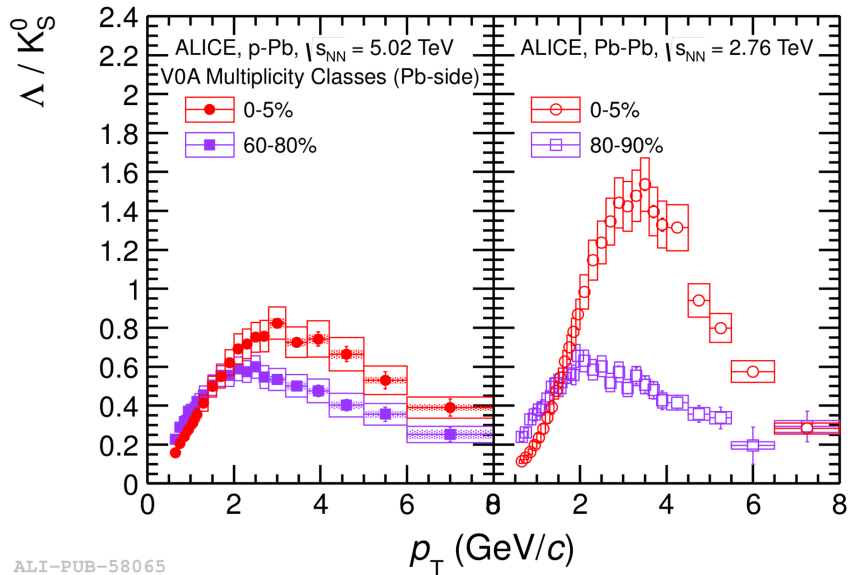
Figure 1.11: \Lambda/K_S^0 ratio obtained with the ALICE experiment in p–Pb collisions at \sqrt{s_{NN}} = 5.02 TeV (left panel) and in Pb–Pb collisions at \sqrt{s_{NN}} = 2.76 TeV (right panel). The results are presented for two multiplicity (centrality) classes for p–Pb (Pb–Pb) collisions [128].
