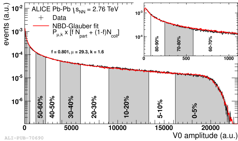
Figure 3.6: Centrality classes of the Pb–Pb collisions in ALICE with the sum of VZERO amplitudes. The negative binomial distribution Glauber fit is shown as the red line [155].
