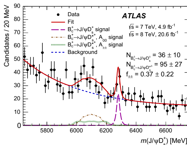
Fig. 3 The mass distribution for the selected J/\psi D_s^+ candidates. The red solid line represents the projection of the fit to the model described in the text. The contribution of the B_c^+ \rightarrow J/\psi D_s^+ decay is shown with the magenta long-dashed line; the brown dash-dot and green dotted lines show the B_c^+ \rightarrow J/\psi D_s^{*+} A_{00} and A_{\pm\pm} component contributions, respectively; the blue dashed line shows the background model. The uncertainties of the listed fit result values are statistical only
