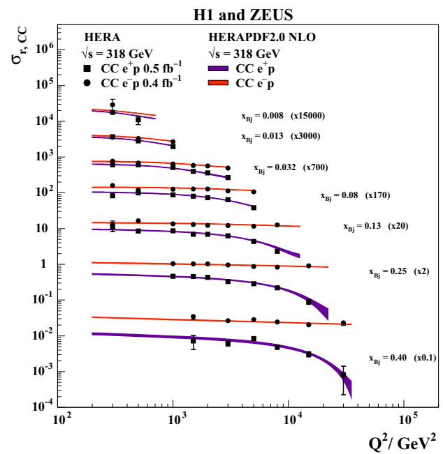
Fig. 79 The combined HERA data for inclusive CC e^+p and e^-p reduced cross sections at \sqrt{s} = 318 GeV with overlaid predictions of HERAPDF2.0 NLO. The bands represent the total uncertainties on the predictions
