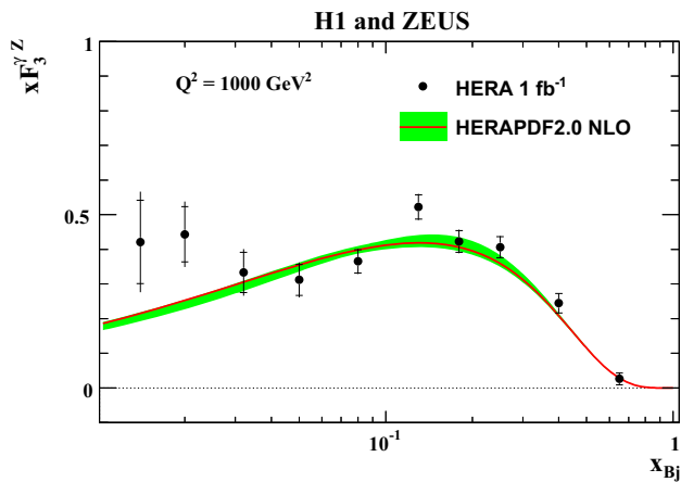
Fig. 78 The structure function x F_3^{\gamma Z} averaged over Q^2 \geq 1000 GeV 2 at the scale Q^2 = 1000 GeV 2 together with the prediction from HERAPDF2.0 NLO. The band represents the total uncertainty on the prediction
