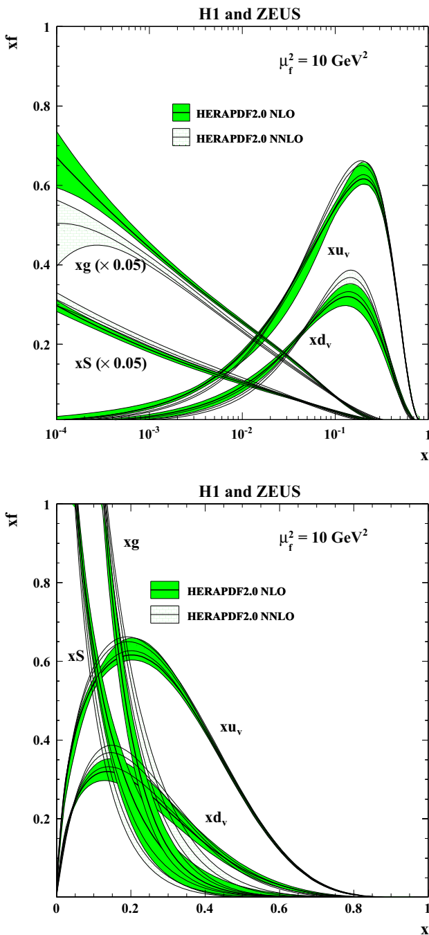
Fig. 25 The parton distribution functions xu_v, xd_v, xS = 2x(\bar{U} + \bar{D}) and xg of HERAPDF2.0 NLO at \mu_f^2 = 10 \text{ GeV}^2 compared to those of HERAPDF2.0 NNLO on logarithmic (top) and linear (bottom) scales. The bands represent the total uncertainties
