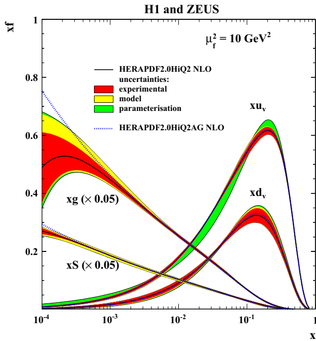
Fig. 52 The parton distribution functions xu_v , xd_v , xS = 2x(\bar{U} + \bar{D}) and xg of HERAPDF2.0 NLO at \mu_f^2 = 10 \text{ GeV}^2 with Q_{\text{min}}^2 = 3.5 \text{ GeV}^2 (top) and of HERAPDF2.0HiQ2 NLO with Q_{\text{min}}^2 = 10 \text{ GeV}^2 (bottom). The gluon and sea distributions are scaled down by a factor of 20. The experimental, model and parameterisation uncertainties are shown. The dotted lines represent HERAPDF2.0AG NLO and HERAPDF2.0AG HiQ2 NLO
