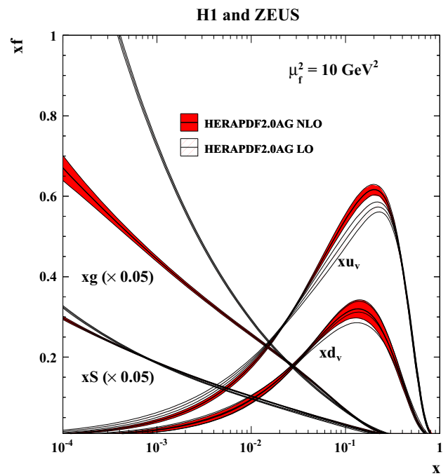
Fig. 26 The parton distribution functions xu_v, xd_v, xS = 2x(\bar{U} + \bar{D}) and xg of HERAPDF2.0AG LO at \mu_f^2 = 10 \text{ GeV}^2 compared to those of HERAPDF2.0AG NLO. The bands represent the experimental uncertainties only
