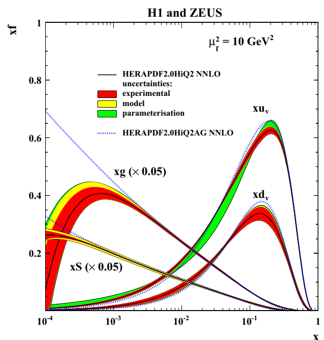
Fig. 53 The parton distribution functions xu_v , xd_v , xS = 2x(\bar{U} + \bar{D}) and xg of HERAPDF2.0 NNLO at \mu_f^2 = 10 \text{ GeV}^2 with Q_{\text{min}}^2 = 3.5 \text{ GeV}^2 (top) and of HERAPDF2.0HiQ2 NNLO with Q_{\text{min}}^2 = 10 \text{ GeV}^2 (bottom). The gluon and sea distributions are scaled down by a factor of 20. The experimental, model and parameterisation uncertainties are shown. The dotted lines represent HERAPDF2.0AG NNLO and HERAPDF2.0AG HiQ2 NNLO
