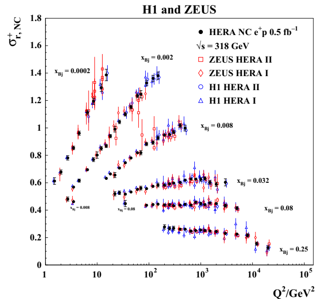
Fig. 4 The combined HERA data for the inclusive NC e^+p reduced cross sections as a function of Q^2 for six selected values of x_{\text{Bj}} compared to the individual H1 and ZEUS data. The individual measurements are displaced horizontally for better visibility. Error bars represent the total uncertainties. The two labelled entries at x_{\text{Bj}} = 0.008 and 0.08 come from data which were taken at \sqrt{s} = 300 GeV and y < 0.35 and were translated to \sqrt{s} = 318 GeV, see Sect. 4.1
