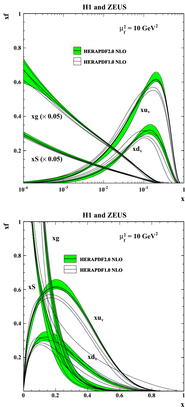
Fig. 47 The parton distribution functions xu_v , xd_v , xS = 2x(\bar{U} + \bar{D}) and xg of HERAPDF2.0 NLO at \mu_f^2 = 10 \text{ GeV}^2 compared to those of HERAPDF1.0 on logarithmic ( top ) and linear ( bottom ) scales. The bands represent the total uncertainties
