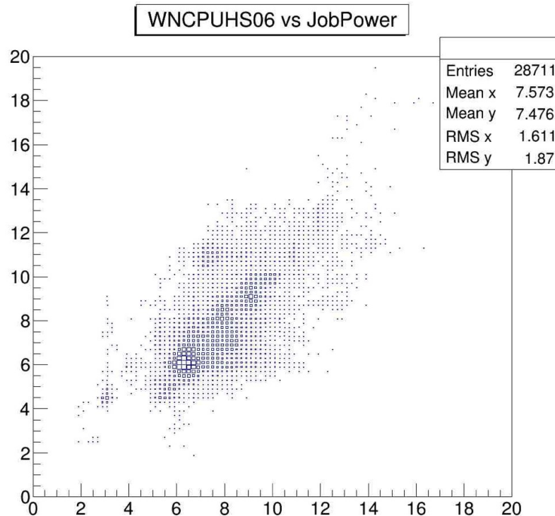
Figure 3. Machine power as calculated by the pilots compared to the power calculated by the simulation jobs, for a single production
