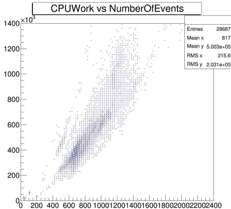
Figure 2. CPU work vs number of events produced by each simulation job, for a single production
