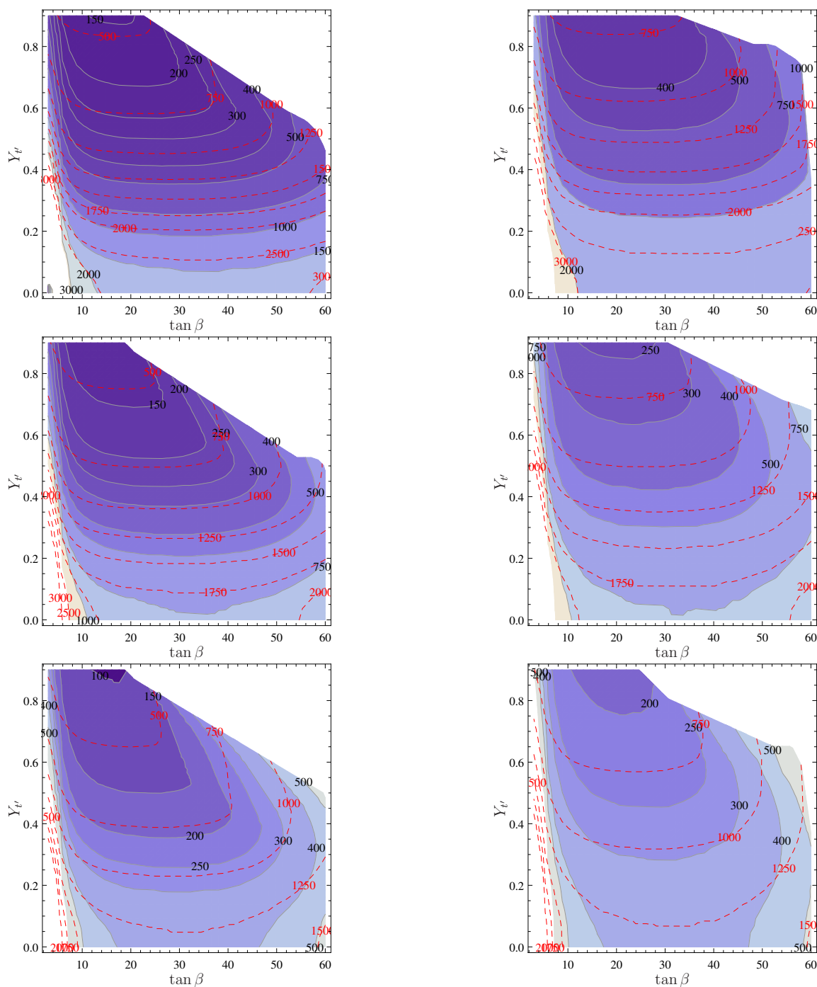
Figure 14. Contours of overall fine-tuning \Delta in the (\tan\beta, Y_{t'}) -plane demanding a Higgs mass m_h = 128 GeV (top), m_h = 125 GeV (middle), and m_h = 122 GeV (bottom) for the UV complete variant of the model. We fixed here M = 10^7 GeV and M_{V'} = 0.5 TeV (left column), respectively, M_{V'} = 1.0 TeV (right column). The red dashed lines indicate the gluino mass in GeV.
