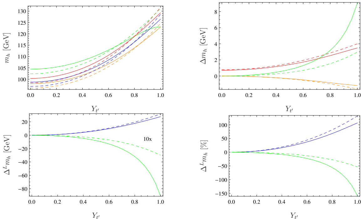
Figure 10. The plots show the same results as in figure 8 for smaller M_A^2 = 10^5 \text{ GeV}^2 . We put T_{t'} = T_u = 0 , and \tan \beta = 3 . The dashed lines are for B_{T'} = 0 , while the full ones correspond to B_{T'} = (1.5 \text{ TeV})^2 .
