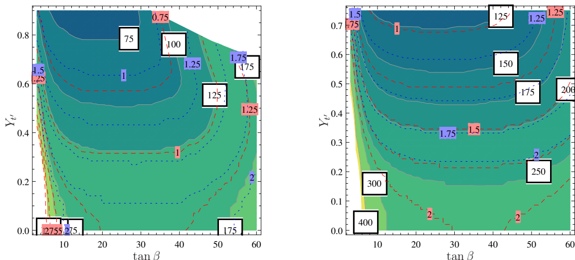
Figure 17. Contours of constant \Lambda (grey), the lightest top-squark mass (small-dashed blue lines) and gluino mass (dashed red lines) in the (\tan \beta, Y_{t'}) -plane demanding a Higgs mass m_h > 122 GeV. All contours are given in units of TeV. On the left side the UV complete model is shown, on the right the model with only vectorlike tops. We fixed M = 10^7 GeV.
