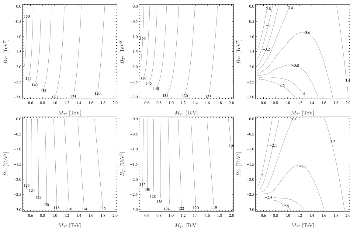
Figure 11. Contour lines of constant m_h at one- (left) and two-loop (middle) in the (M_{T'}, B_{T'}) plane. The plots on the right column show the size of the two-loop corrections involving vectorlike states. The plots in the first row are for Y_{t'} = 1.0 with T_{t'} = 0 and in the second for Y_{t'} = 0.7 with T_{t'} = 1400 GeV .
