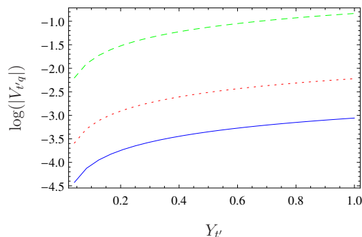
Figure 4. Absolute size |V_{t'q}| of the CKM entries between the vectorlike top states and the SM down quarks q = u, s, b . The colour code is |V_{t'd}| (full blue), |V_{t's}| (dotted red), and |V_{t'b}| (dashed green). We fixed here M_{T'} = 1 TeV.
