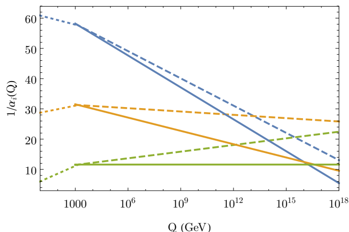
Figure 1. Running of the gauge couplings ( \alpha_i^{-1}(Q) , i = 1, 2, 3 , at 1-loop). The dashed lines belong to the minimal vectorlike top model and the full lines to the UV-completed model. The dotted lines represent the SM-only running up to M_{\text{SUSY}} = 1500 GeV.
