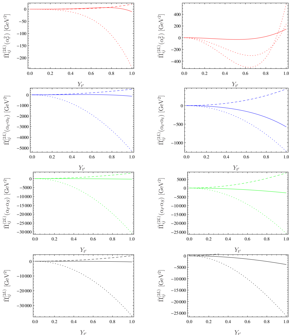
Figure 7. Two-loop contributions the Higgs mass matrix involving vectorlike (s)quark. We used here M_{T'} = 1.0 TeV and put all soft-mass terms to 1.5 TeV. On the left, we set T_{t'} = 0 , on the right T_{t'} = 2.0 TeV \cdot Y_{t'} . Dashed lines are for the (1,1) element, full lines for the (2,2) one, and dotted lines for the off-diagonal contribution. In the first three rows we plot the individual contributions O(\alpha_{t'}^2) , O(\alpha_{t'}\alpha_t) , O(\alpha_{t'}\alpha_S) , while the last row shows the sum of all contributions.
