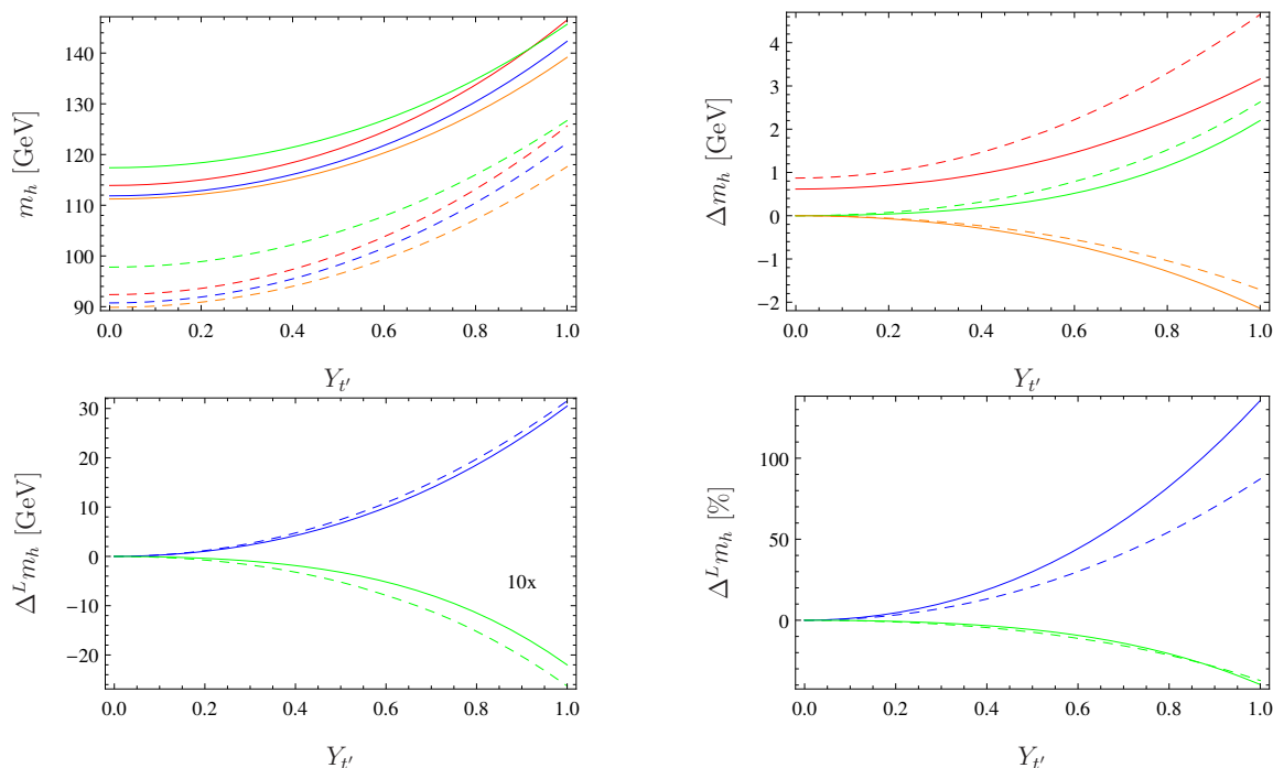
Figure 8. Top left: light Higgs mass as function of Y_{t'} . The red line corresponds to the effective potential calculation at one-loop, orange is the one-loop corrections with external momenta but neglecting the new threshold correction stemming from vectorlike states, blue is the full one-loop calculation including the momentum dependence and all thresholds, and green includes the dominant two-loop corrections together with the full one-loop correction. Top right: impact of the threshold corrections (red), the momentum dependence at one-loop (orange) and the two-loop corrections (green), given as the difference \Delta m_h = m_h - m_h(1L, p^2 \neq 0, \text{all thresholds}) . Note: this plot shows only contributions stemming from the new vectorlike-top sector. Bottom left: absolute size of the one- (blue) and two-loop (green) corrections stemming from the vectorlike states. Note, for better readability we re-scaled the two-loop corrections by a factor of 10. Bottom right: relative importance of the one- (blue) and two-loop (green) corrections normalized to the size of the purely MSSM-like corrections. The full lines are for \tan\beta = 10 and the dotted one are for \tan\beta = 2 . We used here M_{T'} = 1.0 TeV, B_{T'} = 0 .
