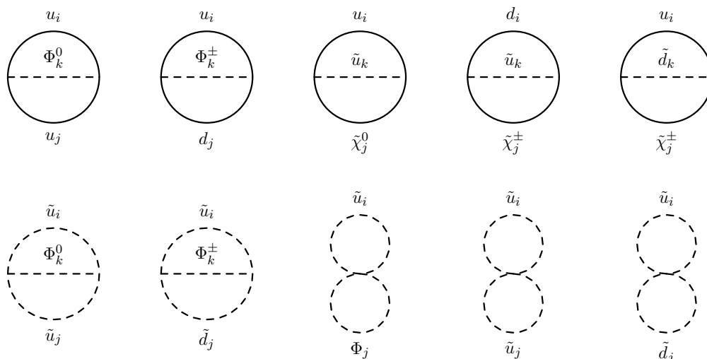
Figure 6. Two-loop diagrams giving contributions to the effective potential O(\alpha_t^2) , O(\alpha_{t'}^2) , and O(\alpha_t \alpha_{t'}) . Here, \Phi^0 = \{h, H, G^0, A^0\} , \Phi^\pm = \{H^\pm, G^\pm\} , \Phi = \{\Phi^0, \Phi^\pm\} . The index ranges are: \Phi(1, 2) ; \tilde{\chi}^0(1 - 4) ; \tilde{\chi}^\pm(1, 2) ; u(1 - 4) ; d(1 - 3) ; \tilde{u}(1 - 8) ; \tilde{d}(1 - 6) .
