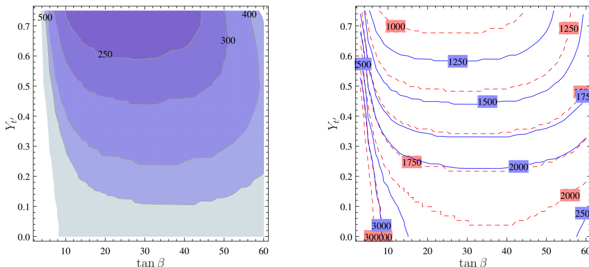
Figure 16. Contours of the overall fine-tuning \Delta (left) and the mass of the lightest up-squark (right, full blue lines) and gluino (right, dashed red lines) in the (\tan \beta, Y_{t'}) -plane demanding a Higgs mass m_h > 122 GeV for the variant of the model without spectator fields. We fixed here M = 10^7 GeV.
