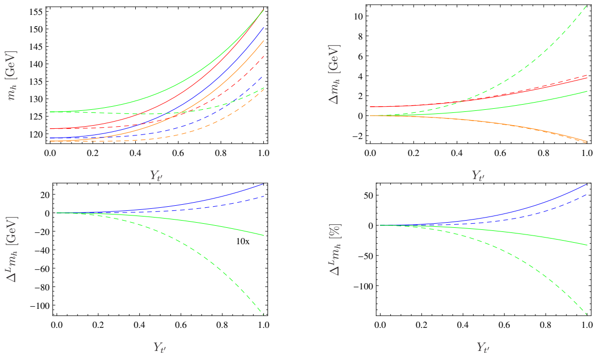
Figure 9. The plots show the same results as in figure 8 when including non-vanishing T_{t'} . We used T_{t'} = 2.0 \text{ TeV} \cdot Y_{t'} , \tan \beta = 5 and T_{u,33} = -2500 \text{ GeV} . The full lines are for B_{T'} = 0 , while the dotted ones correspond to B_{T'} = (1.5 \text{ TeV})^2 .
