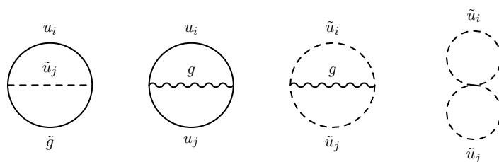
Figure 5. Two-loop diagrams giving contributions to the effective potential O(\alpha_t \alpha_s) and O(\alpha_{t'} \alpha_s) . Here, the indices of up-quark generations ( u_i ) run from 1 to 4, and those of up-squark generations ( \tilde{u}_i ) from 1 to 8.
