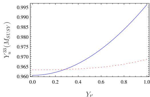
Figure 3. Running top Yukawa coupling ( Y_u^{33} ) at the SUSY scale as function of Y_{t'} for two different values of M_{T'} : 1.0 TeV (blue) and 3.0 TeV (dotted red).
