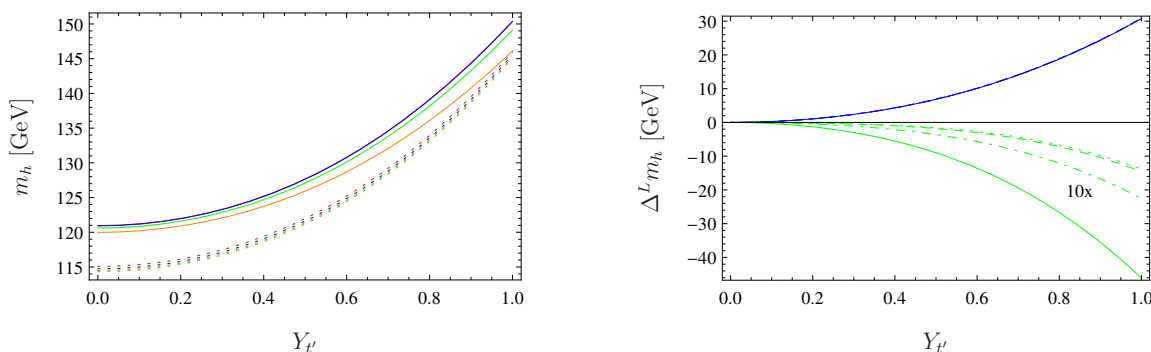
Figure 12. On the left: the light Higgs mass m_h as function of Y_{t'} . Here, we used different values for M_3 : 1 TeV (red), 2 TeV (blue), 3 TeV (green), 4 TeV (orange). The full lines are the two-loop results, the dotted ones the one-loop. On the right the absolute size of the one- (blue) and two-loop (green) corrections involving vectorlike states. The line coding is dashed, dotted, dot-dashed, full for increasing M_3 .
