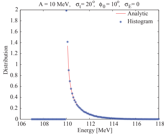
Figure 1: Energy distribution after the PETS for a beam with initial energy E_0 = 120 MeV and a maximum loss of A = 10 MeV. The blue dots are generated in a simulation with 100000 particles and the red line is the result from Eq. 8.
