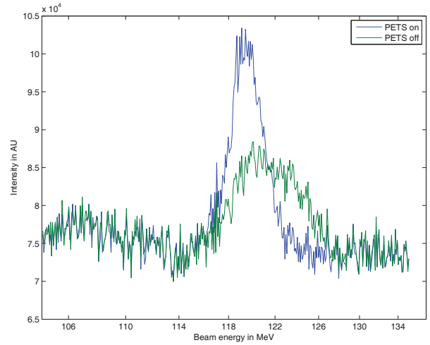
Figure 3: The energy spread of the beam on the spectrometer screen with PETS ON (blue) and OFF (green). Note that the beam energy is higher but the profile is wider in the case of PETS OFF.
