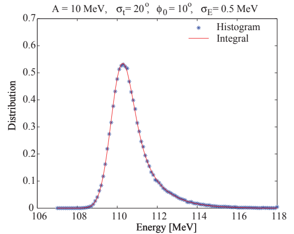
Figure 2: Energy distribution after the PETS for a beam with initial energy E_0 = 120 MeV and maximum loss of A = 10 MeV. Here the initial rms energy spread was taken to be 0.5 MeV. The blue dots are generated in a simulation the red line is the result of Eq. 11.
