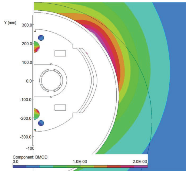
Figure 4: Fringe field outside the cryostat at the design field.
