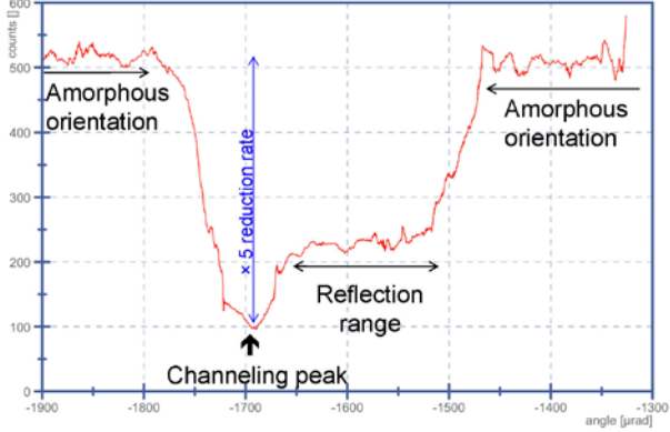
Figure 3: Nuclear loss rate seen by a scintillator telescope downstream of the crystal as a function of crystal orientation angle, revealing the narrow channeling and (wide-acceptance) volume reflection regimes (Courtesy W. Scandale).
