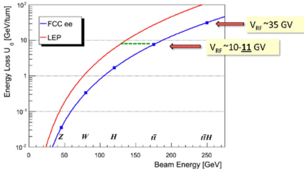
Figure 5: Energy loss per turn as a function of beam energy for LEP and for FCC-ee , translating into a minimum RF voltage required [29].
