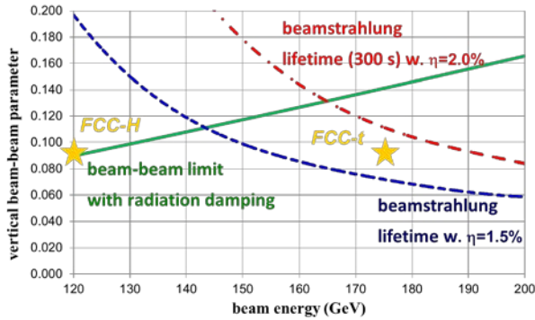
Figure 6: Limits due to classical beam-beam effect and due to beamstrahlung, with two different values for the energy acceptance, as a function of beam energy [35].
