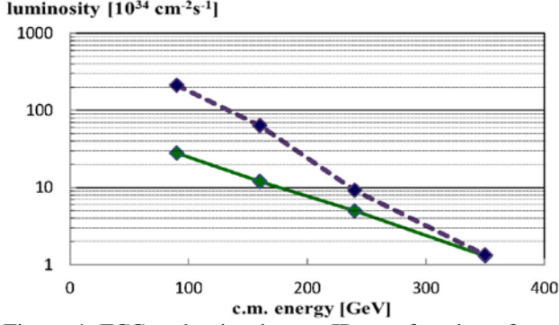
Figure 4: FCC-ee luminosity per IP as a function of c.m. energy. Both the baseline (solid) [25] and an improved collision scheme (dashed) [26] are presented.
