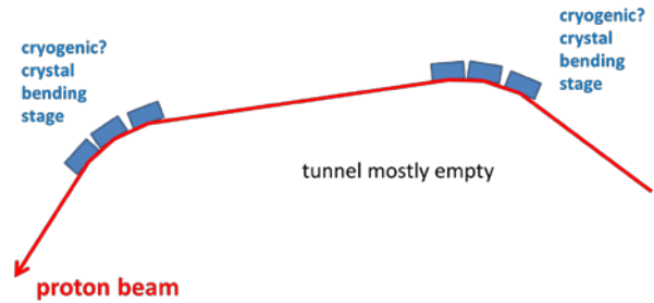
Figure 8: Schematic of a circular crystal collider.
