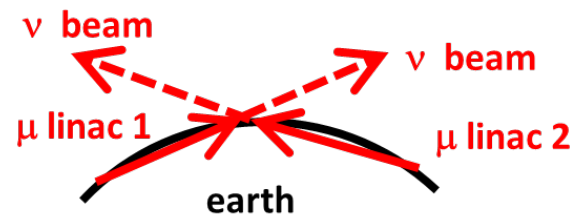
Figure 10: Minimizing the neutrino radiation impacting the earth for a linear muon collider.
