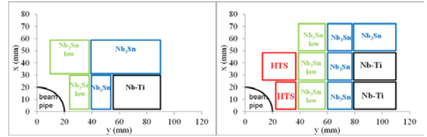
Figure 2: Conceptual designs of 15 or 16 T (left) and 20-T dipole magnets (right) [19]. Only a quarter of one magnet is shown.
