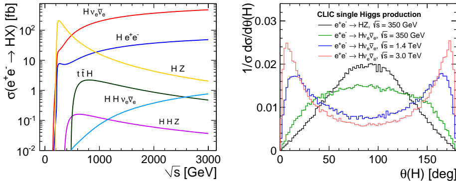
Fig. 1. Left: Cross section as a function of centre-of-mass energy for various Higgs production processes available at CLIC. Taken from [2]. Right: Polar angle of the Higgs produced in Higgsstrahlung and vector–boson fusion events.
