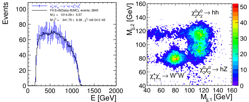
Fig. 5. Left: Reconstructed energy spectrum from slepton decays. Right: Reconstructed di-jet masses from gaugino decays. Both taken from [2].
