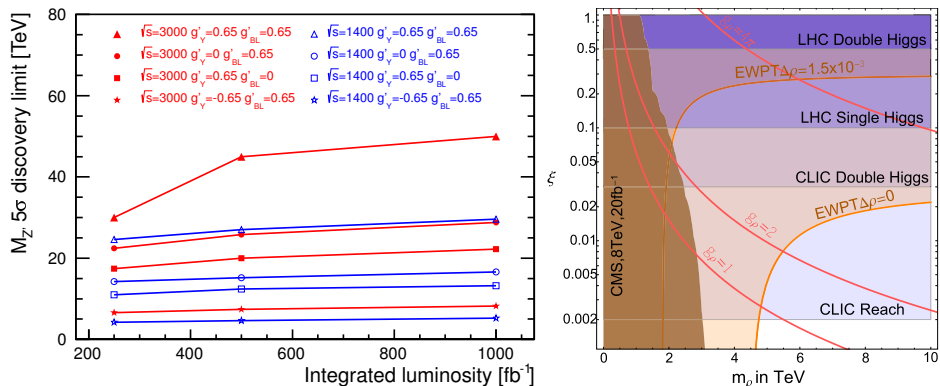
Fig. 7. Left: Z' mass 5\sigma discovery limit as a function of integrated luminosity, for different BSM models. Taken from [21]. Right: Constraints and prospects for ruling out a composite Higgs boson. For more details, see [21]. Taken from [24].
