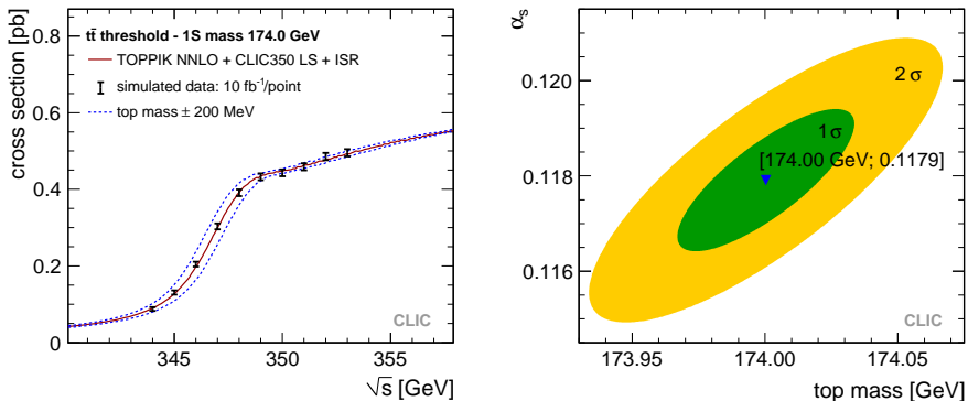
Fig. 4. Left: Cross section as a function of centre-of-mass energy for t\bar{t} production. Right: Correlation between the top mass and \alpha_s , the strong coupling constant. Both taken from [22].
