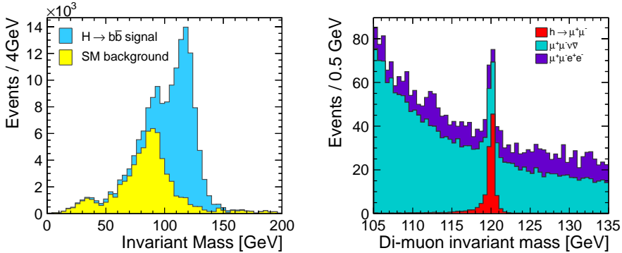
Fig. 2. Left: Reconstructed, selected b\bar{b} invariant mass peak in the H \rightarrow b\bar{b} decay channel. Right: Reconstructed, selected di-muon invariant mass peak in the H \rightarrow \mu^+\mu^- decay channel. Both taken from [2].
