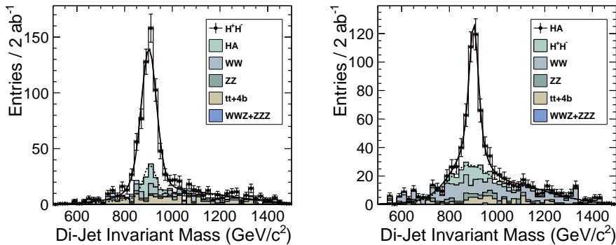
Fig. 6. Heavy Higgs bosons produced at \sqrt{s} = 3 TeV, which are almost degenerate in mass. Left: The charged H^+H^- , decaying to t\bar{t} pairs. Right: The neutral HA , decaying to b\bar{b} pairs. Both taken from [2].
