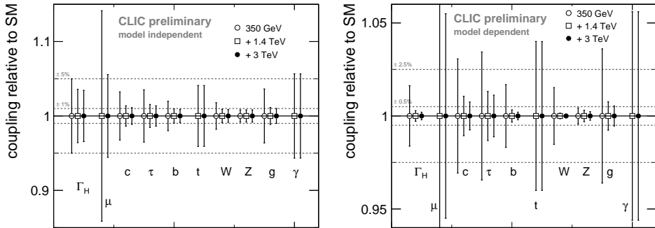
Fig. 3. Illustration of the achievable precision on the Higgs couplings and decay width after three successive CLIC energy stages. Left: For a model-independent combined fit. Right: For a model-dependent combined fit. Results at \sqrt{s} = 1.4 TeV and 3 TeV are scaled to reflect -80\% electron beam polarisation.
